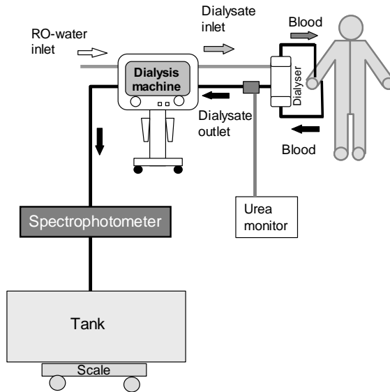
Fig. 18. The clinical set up in Paper II.
