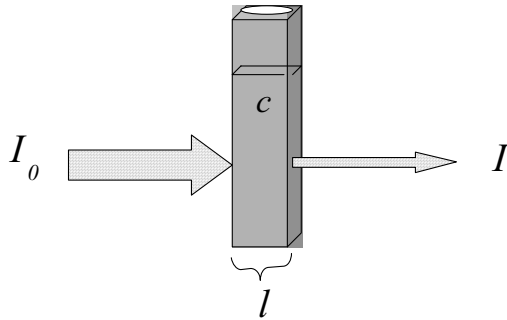
Figure 9. A cuvette containing solution. The absorbance is dependent on the path length l , the concentration of solutes c , and the millimolar absorptivity by the solute, \epsilon
