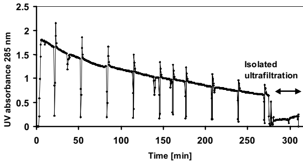
Figure 26. Isolated ultra filtration after dialysis treatment (i.e. no dialysis fluid trough the dialyser). A few alams is also seen at 40, 140 and 160 min corresponding to blood pump stops.
