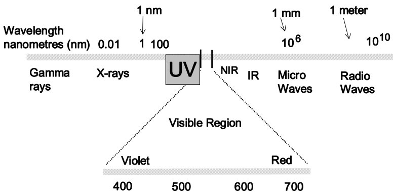
Figure 8. Electromagnetic spectrum from the shortest wavelength, gamma radiation to longest, radio waves.
