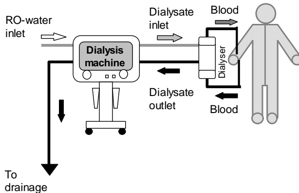
Figure 1. Schematically set up of a dialysis treatment
