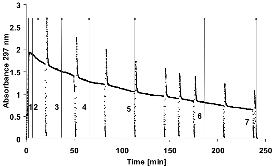
Figure 24. AUCa^{297} divided in sub areas according to the samples taken from the tank, 1 to 7 in the figure. Those sub areas were then correlated to the total removal of the studied solutes.
