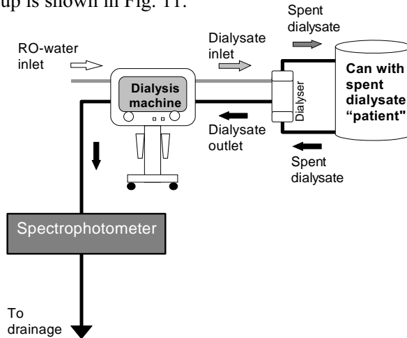
Figure 11. Set up during on-line in vitro tests. The can was filled with spent ultrafiltrate or spent dialysate
