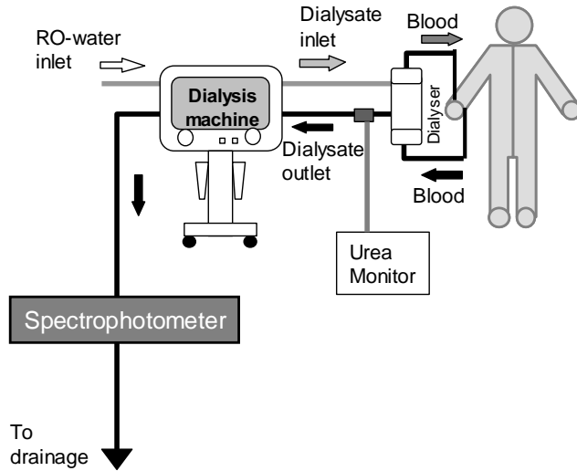
Figure 16. The clinical set up in Paper I. The spectrophotometer and the Urea Monitor 1000 is connected to the drain tube of the dialysis machine
