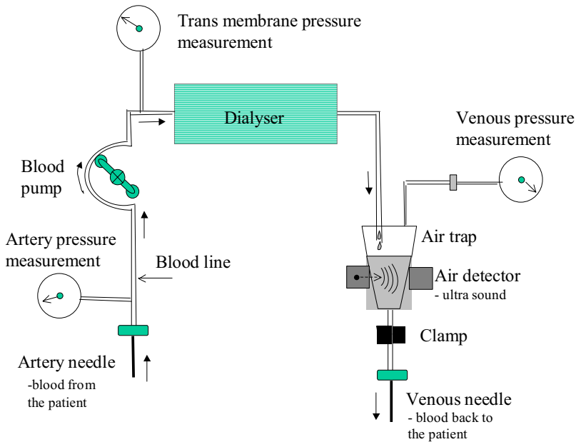
Fig. 2. The blood-part of the dialysis machine schematically
