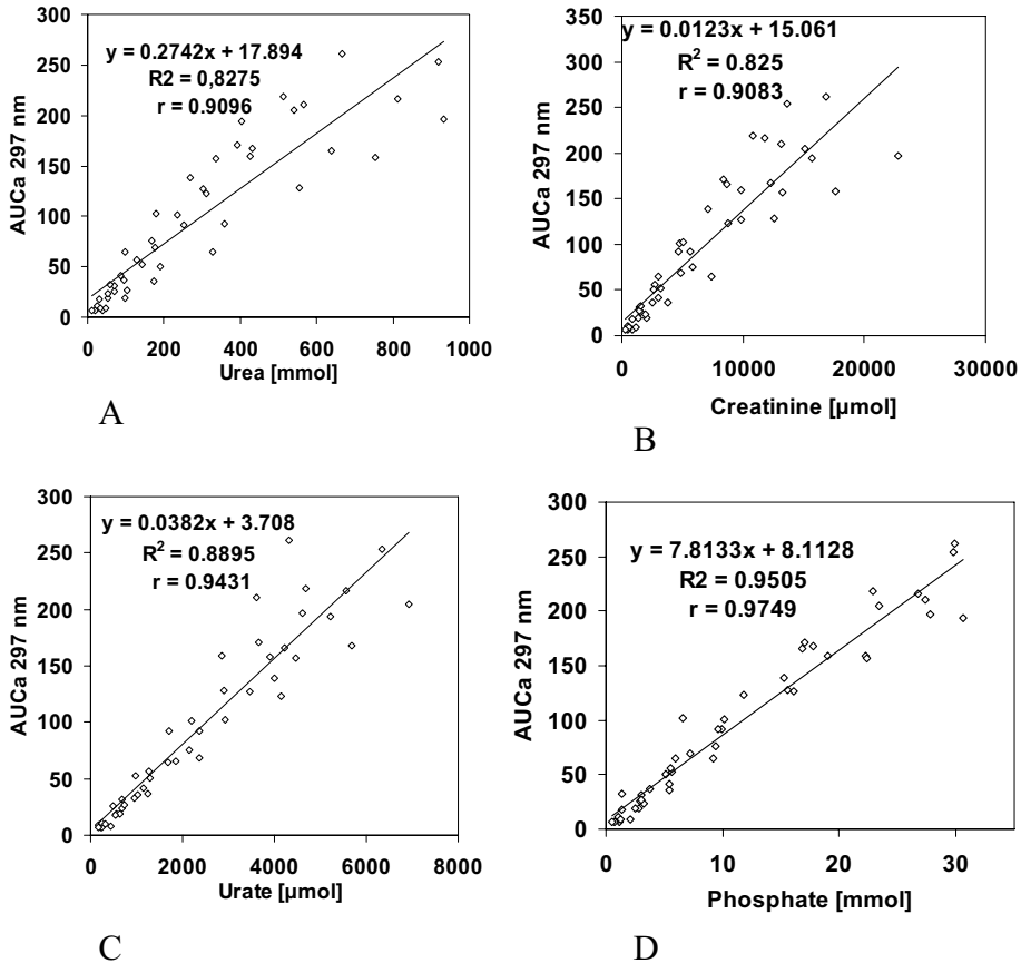
Fig. 25. The correlation between accumulated areas of AUCa^{297} correlated to accumulated total removal of urea (A), creatinine (B), urate (C) and phosphate (D)
