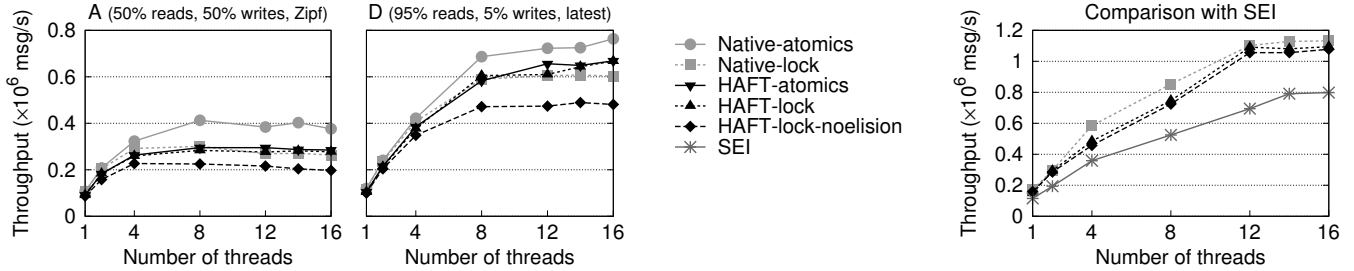
Figure 11: Memcached throughput. Left two graphs: workloads A and D. Right graph: comparison of HAFT and SEI using a mcbuster client, a key range of 1,000, and values of size 128 B (same experimental setup as in [11]).
