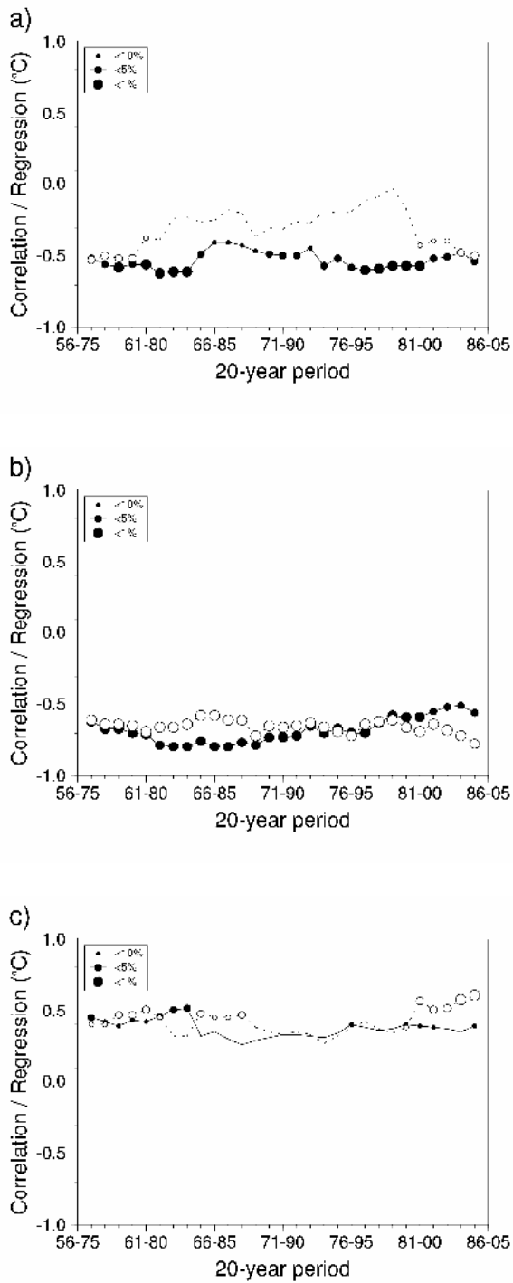
Figure 4. Temporal changes in the magnitude and significance in the correlation between the SAM and near-surface temperatures using a running 20-year window: (a) Amundsen-Scott; (b) Mawson; and (c) Esperanza. Winter data are the solid line and filled circles, summer data the dotted line and open circles.
