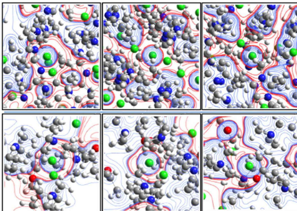
Figure 4. Concentro-spherical shells composed of alternating +/- electrostatic potential regions (light-red/light-blue contours) for the C_{ali}-H\cdots Cl^- interactions of [1](Cl)_2 (upper three panels) and the BUXTOD complex involving tetraalkyl-ammonium cations (lower three panels) at the B97D/cc-pVDZ level (Each three panels denote the +/- electrostatic potential contour maps on the three perpendicular planes with respect to the Cl^- anion. Isodensity surface value: 0.01 au; Isovalue for contour; 0.008 au. (Cl: green, O: red, N: blue, C: dark grey, H: light grey).
