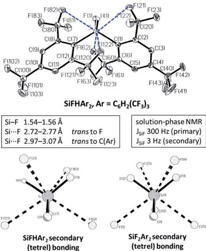
Fig. 11 Crystal structure of SiFHA 2 , Ar = C 6 H 2 (CF 3 ) 3 (top), with secondary (tetrel) bonding shown as dashed bonds and primary bonding (solid lines) and secondary bonding (dashed lines) at Si in SiFHA 2 and SiF 2 Ar 2 (bottom). Secondary (tetrel) Si···F bonds are longer than primary (covalent) Si–F bonds. Secondary bonds trans to F are shorter than those trans to C. Adapted from ref. 57 with permission from Elsevier.
