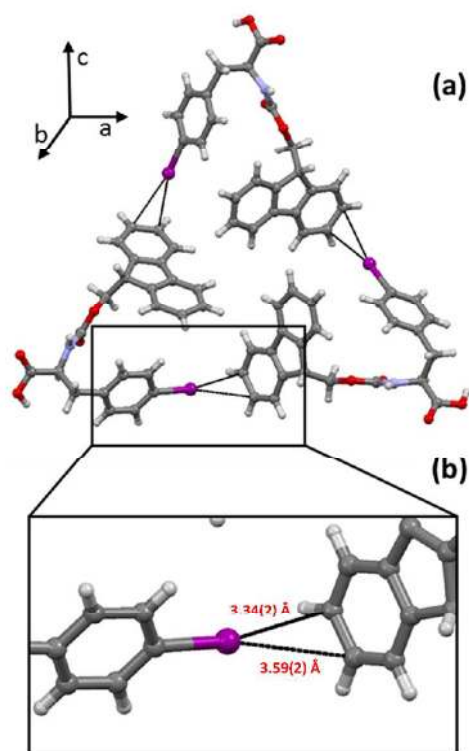
Fig. 4. Single crystal X-ray structure of the Fmoc-4-I-Phe derivative. a) Iodine... \pi interactions lead to the self-assembly of three bent amino acid molecules into a triangular hydrophobic pocket where the fluorenyl rings are confined. b) Magnification of the iodine... \pi interactions involving iodine and one of the bonds of the fluorenyl moiety.
