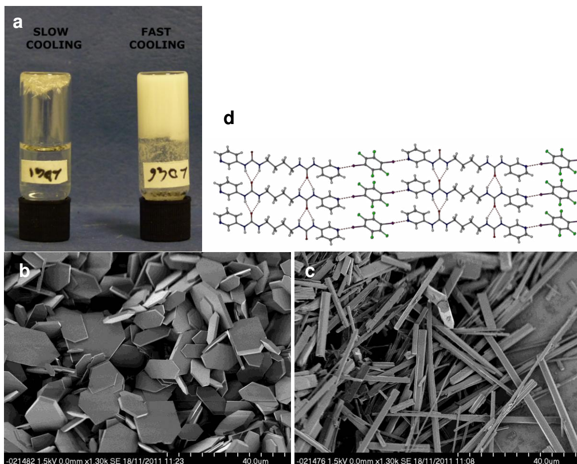
Figure 3 Gel formation by halogen-bonding. (a) Rapid cooling of an equimolar mixture of bis(pyridyl urea) 1 and diiodotetrafluorobenzene in methanol/water (4:1 v/v) results in a robust hydrogel while slow cooling gives a fibrous crystalline precipitate. (b) SEM micrograph of crystalline 1 showing plate-like morphology, (c) SEM micrograph of 1 · 3
