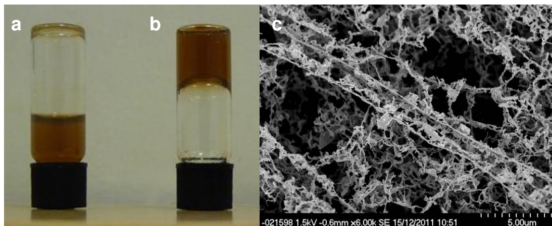
Figure 6 Co-gel formation between halogen-bond acceptor and halogen-bond donor bis(urea)s 1 and 4. (a) Compound 4 in DMSO/water 3:1 does not undergo gelation whereas, (b) in the presence of 1 it forms a co-gel 1·4 in DMSO/water 3:1. (c) SEM micrograph showing the morphology of the 1·4 co-gel.
