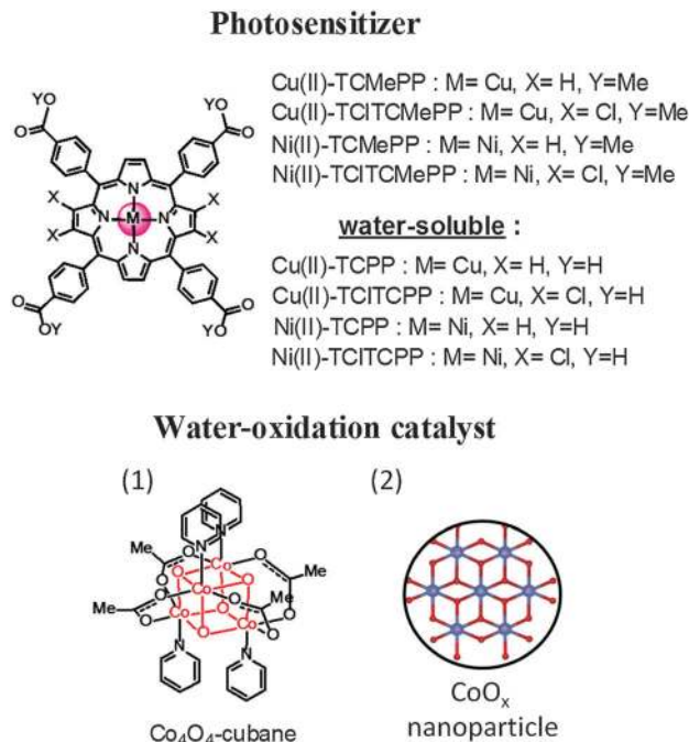
Fig. 1 Chemical structures of Cu(II)- and Ni(II)-porphyrinphotosensitizers and water oxidation catalyst: (1) Co 4 O 4 -cubane, (2) representation of CoO x nanoparticle formed from Co(NO 3 ) 2 pre-catalyst. 7,35,36
