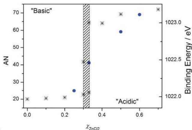
Figure 28. Plots of AN values (calculated by Estager et al. 27 (black stars) and Zn 2p 3/2 binding energies (blue circles) against composition, \chi_{ZnCl_2} , of the [C 8 mim]Cl-ZnCl 2 system. The neutral zone is shown as a shaded region between \chi_{ZnCl_2} = 0.3 and 0.33 (reproduced from Ref. 58).
