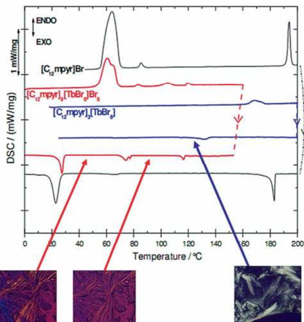
Figure 46. DSC-thermograms of [\text{C}_{12}\text{mpyr}]\text{Br}-\text{TbBr}_3 system, \chi_{\text{TbBr}_3} = 0.10 (in red) and \chi_{\text{TbBr}_3} = 0.25 (in blue) with corresponding POM micrographs, compared to the thermogram of neat [\text{C}_{12}\text{mpyr}]\text{Br} (reproduced from Ref. 299 with permission from Wiley).
