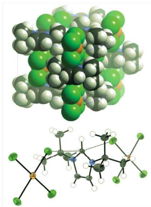
Figure 20. Two views of the crystal structure of [\text{C}'_4\text{Ca'im}]\text{Cl-AuCl}_3 : pseudo -NaCl structure packing in space-filling representation (top), and detail of anion- \pi interactions (bottom). Thermal ellipsoids displayed at 50% probability (reproduced from Ref. 110).
