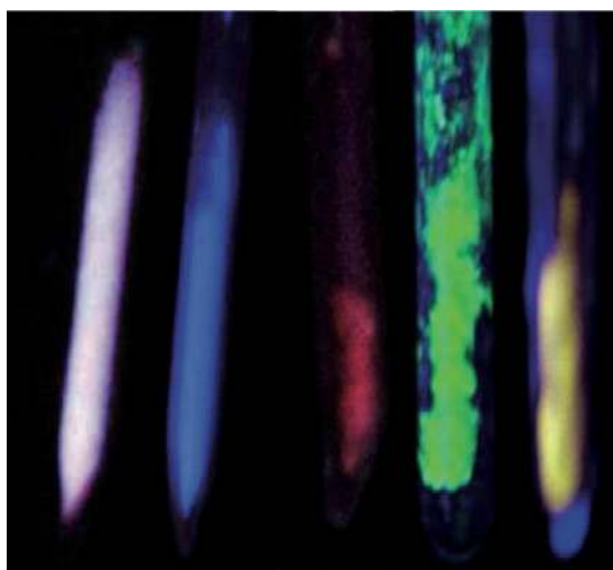
Figure 47. Neat [\text{C}_{12}\text{mim}]\text{Br} (left) doped with various lanthanide bromides under UV light (reproduced from Ref. 297 with permission from Wiley).
