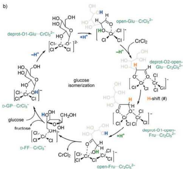
Figure 33. (a) Ab initio determined energy pathway for glucose isomerisation involving mono- (blue) and binuclear (orange) Cr(II) complexes with the carbohydrate in a model MMIM ionic liquid. The red line highlights the path of lowest free energy. (b) The proposed catalytic cycle corresponding catalytic cycle for the isomerisation of glucose in the presence of CrCl 2 in a model MMIM ionic liquid medium. d-FF = d-fructofuranose, d-GP = d-glucopyranose (reproduced from Ref. 220 with permission from Wiley).
