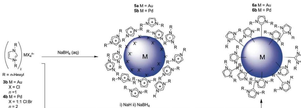
Figure 43. Synthesis of imidazolium and NHC stabilised metal nanoparticles (reproduced from Ref. 110).
