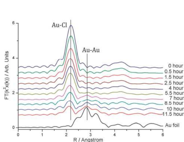
Figure 10. Evolution of the k^2 -weighted pseudo -radial distribution functions in the [C 4 mim][AuCl 4 ] \cdot 4H 2 O system as a function of time of exposure to the X-ray beam. The gradually decreasing peak ca. 2.2 Å, corresponds to the change in Au–Cl coordination number; the gradually increasing peak ca. 2.8 Å reflects increasing Au–Au contact (Reproduced from Ref. 71 with permission from the PCCP Owner Societies).
