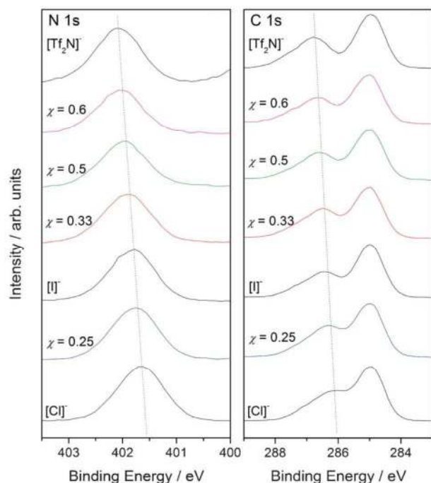
Figure 21. High resolution XP spectra of the N 1s and C 1s regions for four [C 8 mim]Cl-ZnCl 2 ( \chi_{\text{ZnCl}_2} = 0.25, 0.33, 0.50, 0.60 ), compared to [C 8 mim]Cl, [C 8 mim]I and [C 8 mim][NTf 2 ]. All spectra have been charge corrected to C aliphatic 1s = 285.0 eV. (reproduced from Ref. 58).
