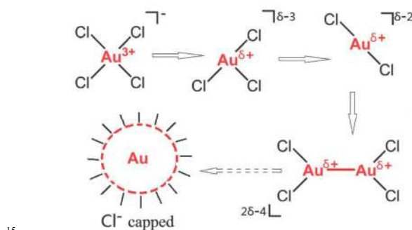
Figure 11. The proposed mechanism of gold nanoparticles formation under synchrotron X-ray irradiation of [C 4 mim][AuCl 4 ] \cdot 4H 2 O; \delta = 0-3 (Reproduced from Ref. 71 with permission from the PCCP Owner Societies).
