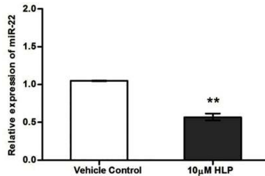
Fig 4. Effect of HLP on miR-22 expression in SK-N-SH cells.
