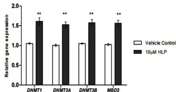
Fig 2. Effect of HLP on gene expression of epigenetic genes in SK-N-SH cells.
