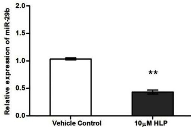
Fig 3. Effect of HLP on miR-29b expression in SK-N-SH cells.
