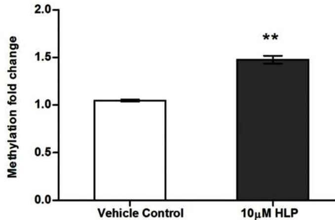
Fig 1. Effect of HLP on global DNA methylation in SK-N-SH cells.
