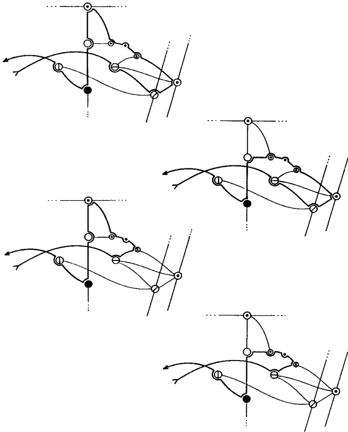
Fig. 8. Four ways of visiting a node as a shadow in G_3 .
