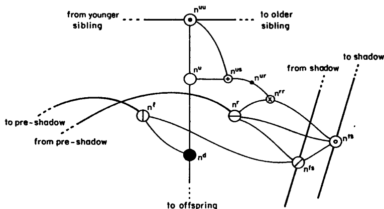
Fig. 6. Internal nodes and edges in G_3 .
