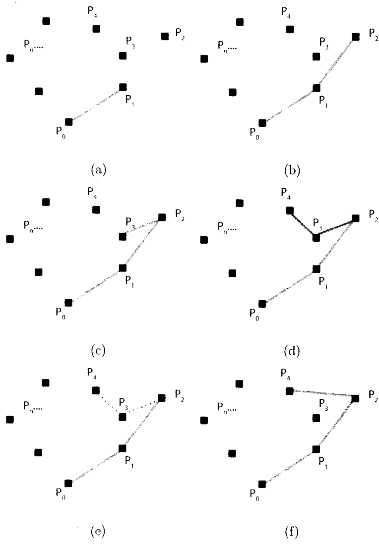
Figure 3. Graham Scan
