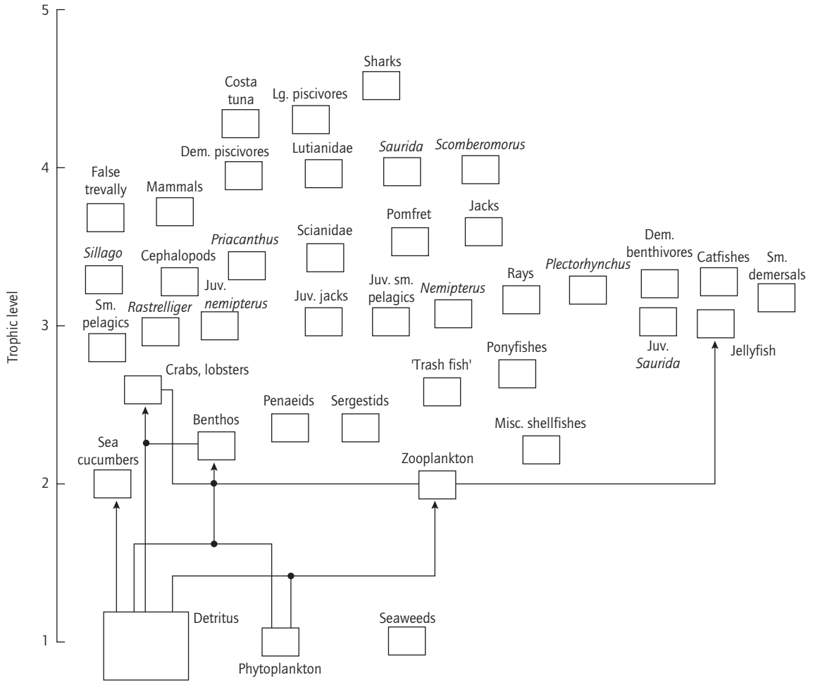
Fig. 10.1 Flow diagram for a trophic model of the Gulf of Thailand. All flows between ecosystem groups are quantified, but only flows exceeding 5 t·km 2 ·year -1 are indicated. The sizes of the boxes are a function of the group biomasses.
