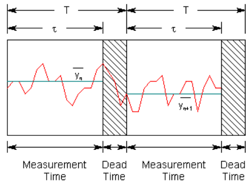
Figure 23. Illustration of dead time between successive measurements.
