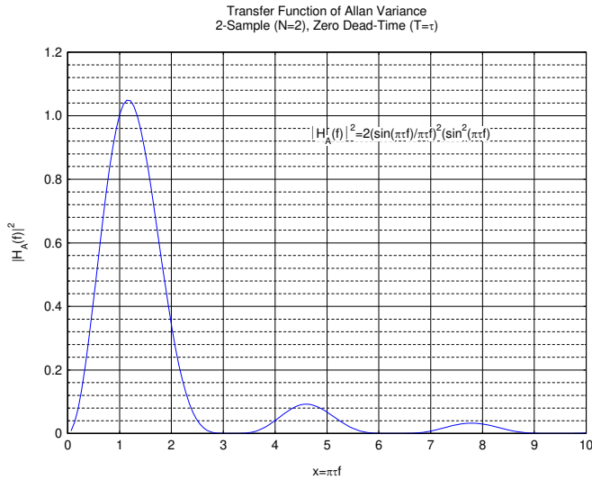
(a) Allan Variance
