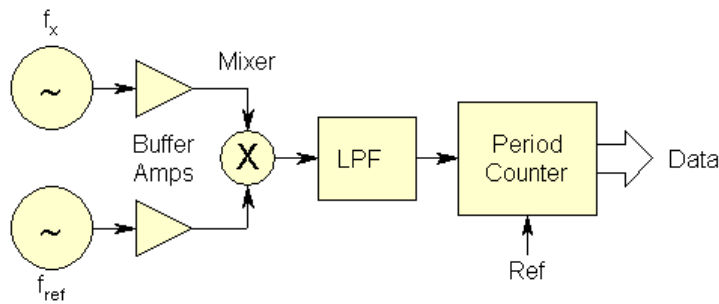
Figure 35. Block diagram of a heterodyne measuring system.
