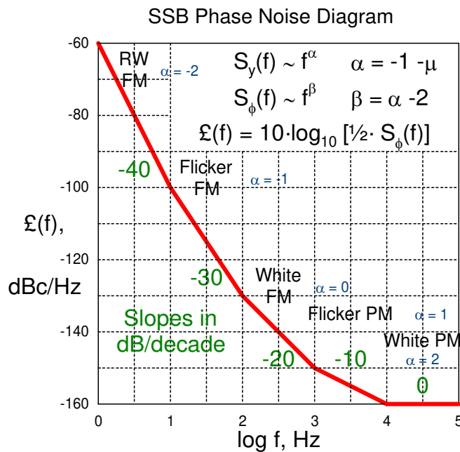
Figure 31. SSB Phase Noise Plot.
