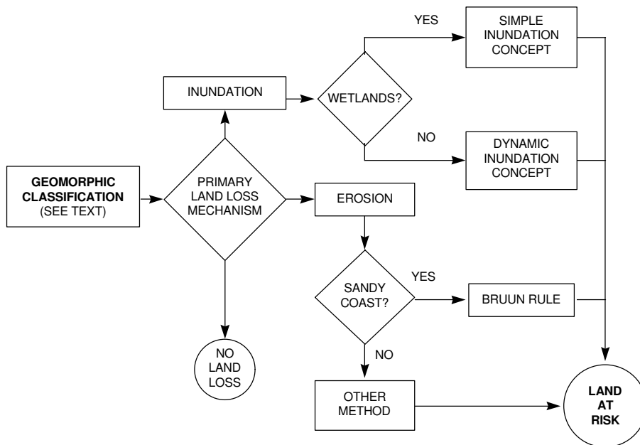
Figure 7.2 Flow-diagram to determine the appropriate method to determine land at risk from erosion or inundation (Nicholls et al., 1995). Wetlands embrace marshes, mangroves, and coral atolls/keys.
