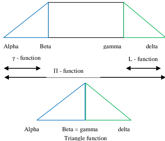
Figure 2. Membership functions
