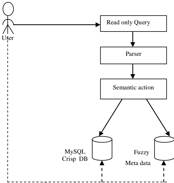
Figure 1: System Architecture
