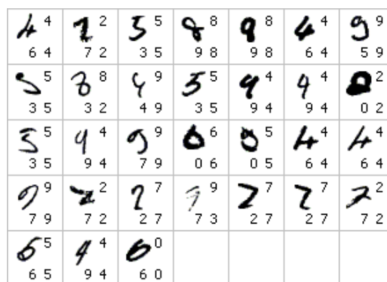
Figure 4: The committee’s miss-classified digits together with the two most likely predictions (bottom, from left to right) and the correct label (top right) according to MNIST.
