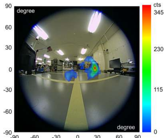
Fig. 7. Compton reconstructed image of a ^{137}\text{Cs} isotope, taken with a prototype Compton camera as shown in Fig. 5. An integration time of 30 s is needed to reconstruct the image for a weak source when the corresponding radiation dose is \approx 6 \mu\text{Sv/h} .
