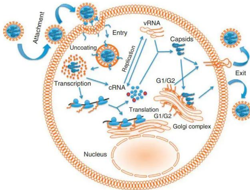
Fig. 2. Hantavirus replication
