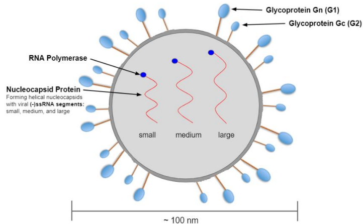
Fig. 1. Hantavirus structure
