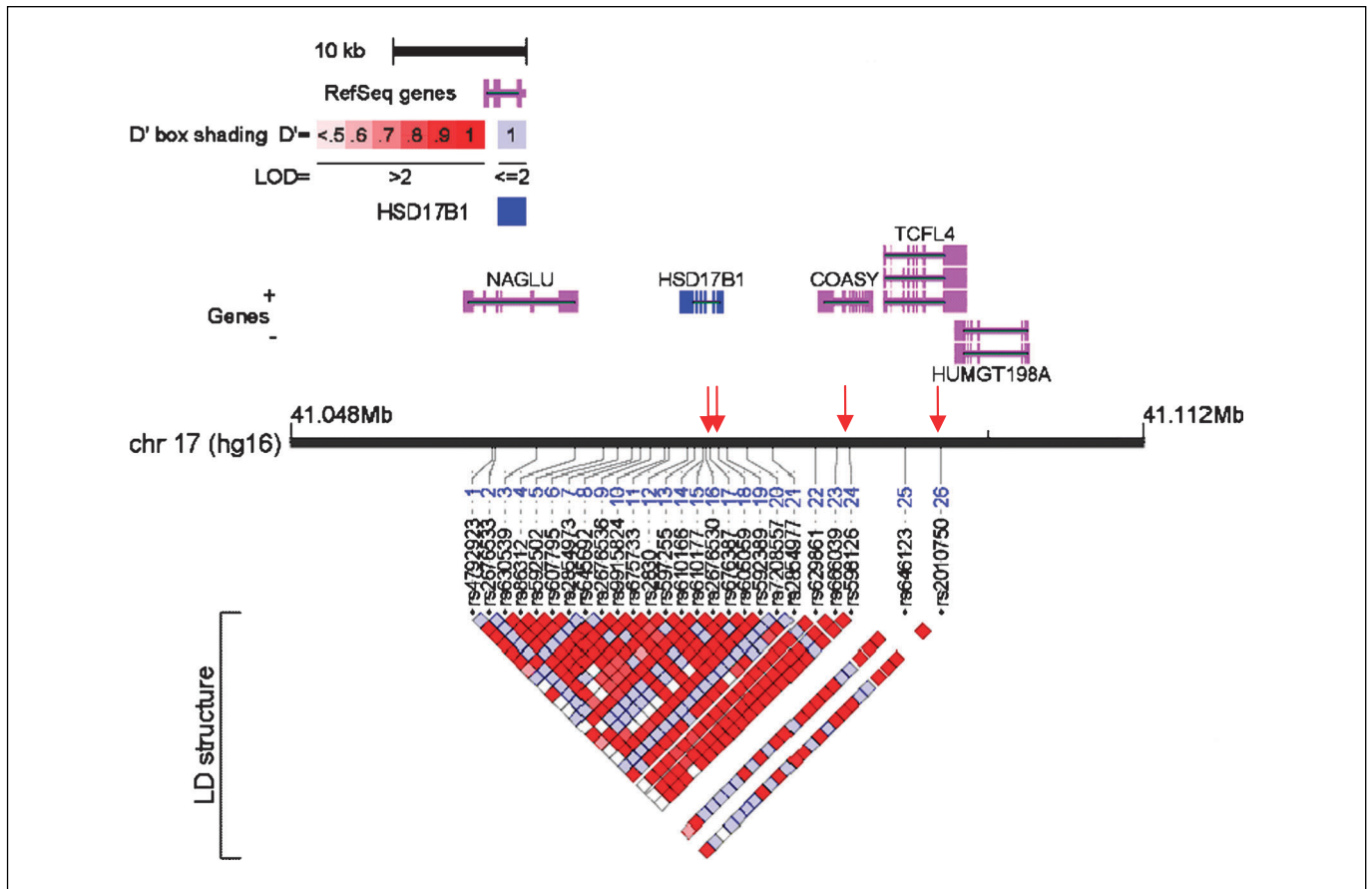
Figure 1. SNPs and linkage disequilibrium structure (among Caucasians) across the HSD17B1 locus. Twenty-six SNPs were selected covering a 42-kb region around HSD17B1 at an average density of one SNP per 1.6 kb. Haplotype tagging SNPs (red arrows).
