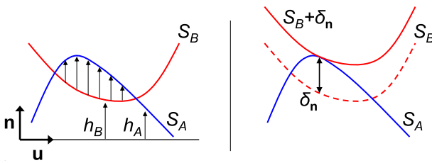
Figure 3: Penetration Depth of Height Fields. Directional penetration depth of surface patches expressed as height difference.
