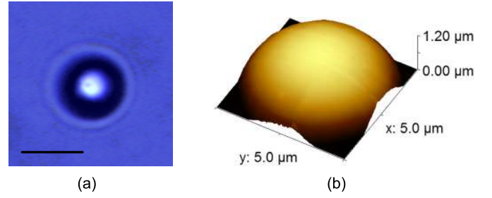
Fig. 5. (a) An optical image of a microsphere under 100 \times optical magnification (the scale bar represents 5 \mu m). (b) An AFM image scan on the microsphere.
