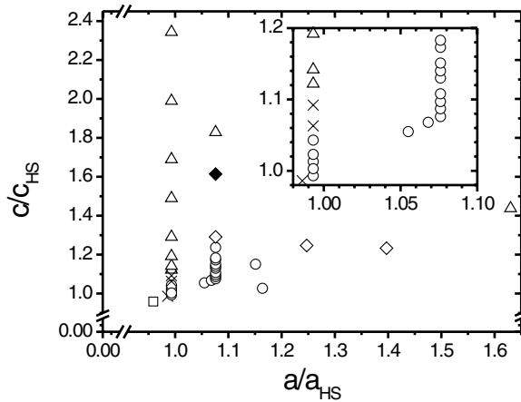
FIG. 3. Crystal phases versus scaled lattice parameters. The open symbols denote the occurrence of a stable phase from the template onwards: hcp ( \circ ), fcc ( \square ), or hexagonally stacked ( \triangle ); crosses ( \times ) indicate hcp(1100) in the third layer and fcc(100) in the tenth layer. The filled diamond indicates a non-CP structure. The open diamonds denote a disordered state in the first layers above the template.
