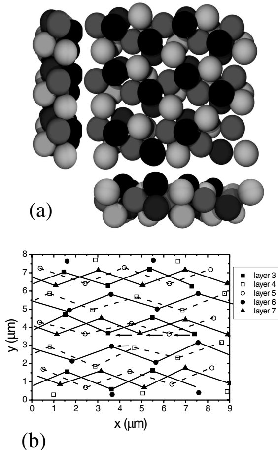
FIG. 4. (a) A reconstruction based on particle coordinates in layers 3 to 7 at an anisotropically stretched template with a/a_{\text{HS}} = 1.076 and an axis ratio of c/c_{\text{HS}}(a/a_{\text{HS}})^{-1} = 1.50 . The image in the middle shows a top view, and the other two the respective side views. Black spheres (diameter drawn to scale) are in layer 7, light gray in layers 3 and 6, and dark gray in layers 4 and 5. (b) A projection of lateral particle coordinates for particles in (a) onto a single layer. Positions indicated with filled symbols have been connected with solid lines and open symbols with dashed lines, which indicates the template-induced alignment. The arrows indicate the shift in particle positions between layers 3, 5, 7, and 9 (= 3) and layers 4 and 6, respectively.
