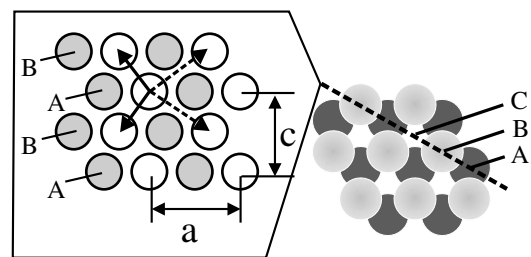
FIG. 1. Right: Particle positions in two successive hexagonally stacked (111) planes with the three stacking possibilities A, B, C indicated. The dashed line indicates the orientation of the perpendicular hcp(110) plane with respect to the (111) planes. Left: A projection of sphere positions in two successive hcp(110) layers. The solid arrows indicate the in-plane nearest-neighbor distances r_1 and r_2 , and the dashed arrows the next-nearest-neighbor distances r_3 and r_4 . The lattice distances a and c are indicated as well.
