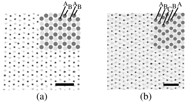
FIG. 2. Confocal images of (a) the 18th layer in a templated hcp ( ABA ) crystal, with the 19th layer vaguely visible as well, and (b) the 10th layer in a dhcp ( ABCBA ) crystal. In the top right corner of both images, spheres have been drawn (not to scale) on the experimentally determined particles positions. Dark gray: lateral coordinates of in-focus particles; light gray: out-of-focus particles. Scale bars are 5 \mu\text{m} .
