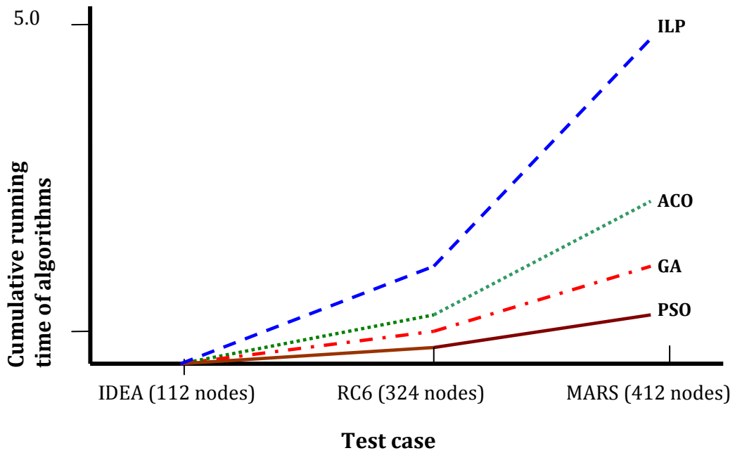
Figure 2. Results of computer simulations for cumulative running time of the algorithms on benchmark problems.
