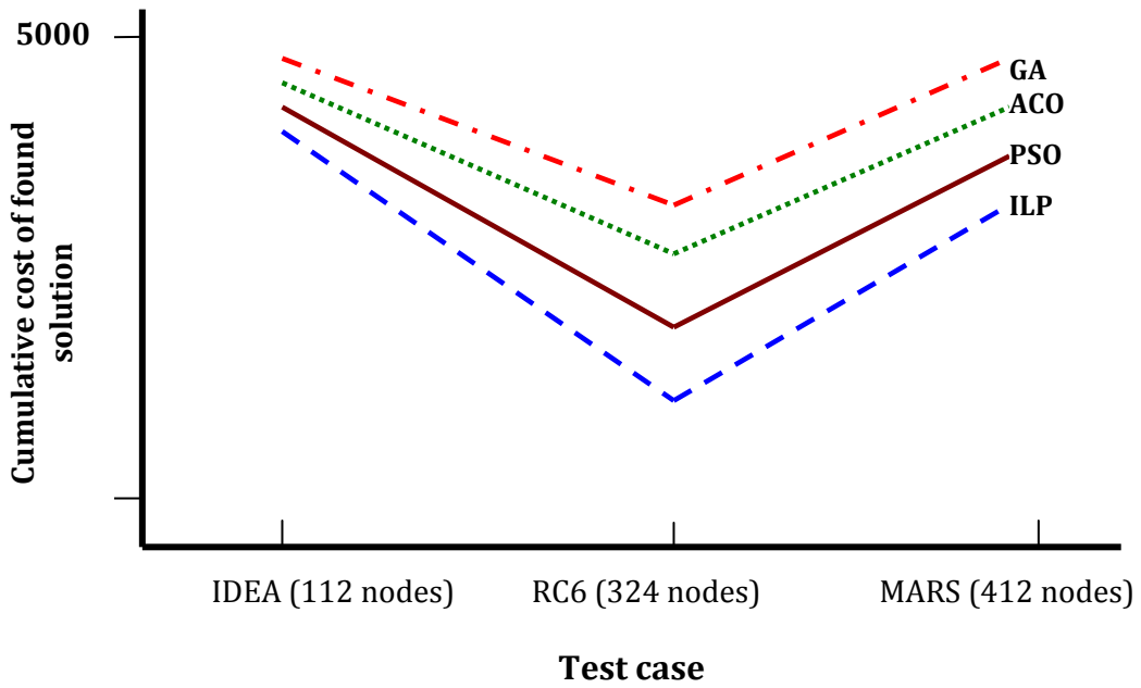
Figure 3. Results of computer simulation for cumulative cost of found solution of different algorithms on different benchmark problems.
