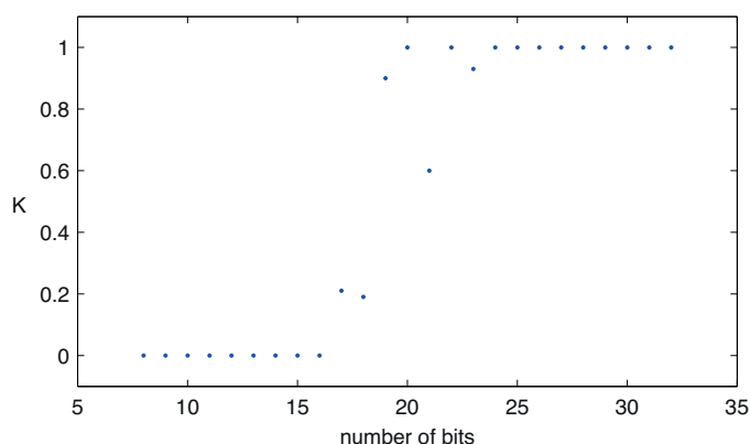
Fig. 8. Values of K as a function of the number of bits in fixed point representation
