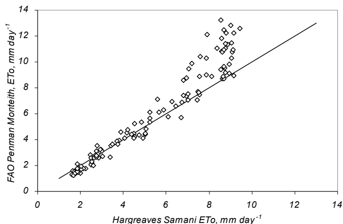
Fig. 1. Relation between ET_0 calculated with the HS equation and the PM for the dry conditions of Abadan, Iran. The Hargreaves Samani equation fails to calculate ET_0 values above 9 \text{ mm day}^{-1} (data kindly provided by Rahimkoob)
