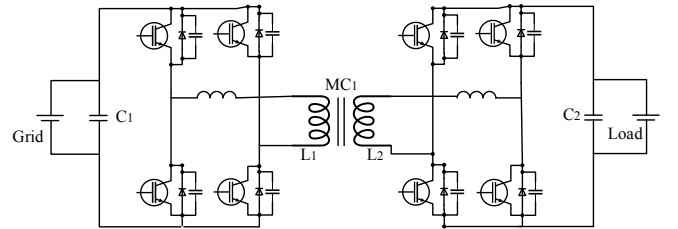
Figure 4. Topology of bidirectional isolated power converter
