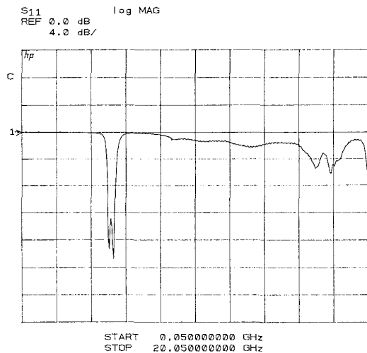
Fig. 9(b) Measured return loss of daisy ring filter
