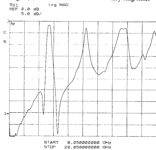
Fig. 10 Measured insertion loss of standard dual-mode ring
