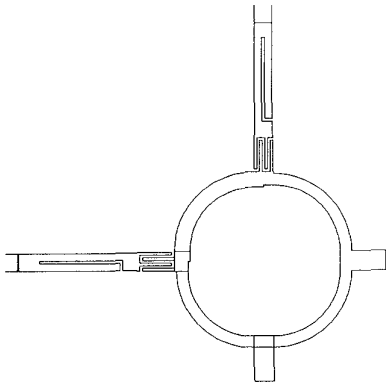
Fig. 1. Spur-line band-stop filter.
