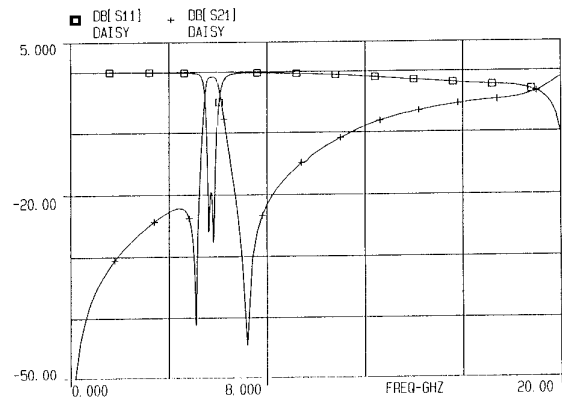
Fig. 8 Simulated response of the daisy ring filter
