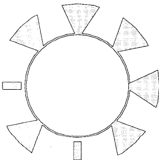
Fig. 6(c) Low pass ring with radial stubs
