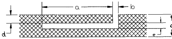
Fig. 1. Spur-line band-stop filter.
