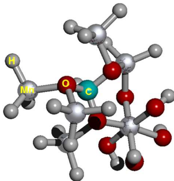
Figure 2. Cell structure of a protonated rhodochrosite crystal. Represented in red the oxygen; silver in color Manganese; in gray color Hydrogen; in light see green color the Carbon. Stoichiometry: CMn_6O_8 . Stoichiometry protonated: CH_{19}Mn_6O_8 .
