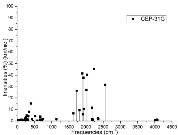
Figure 4. Absorbance spectrum plot as a function of vibrational frequencies of protonated rhodochrosite crystal for UHF-CEP-31G basis set.
