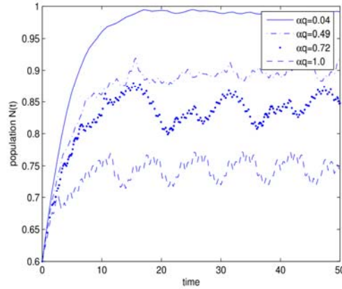
Figure 12: Seasonal harvesting with data3
