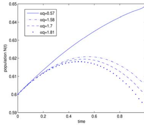
Figure 10: Seasonal harvesting one year solution with data2
