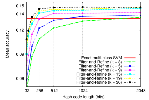
Figure 1: Exact Multi-class SVM vs Filter-And-Refine method
