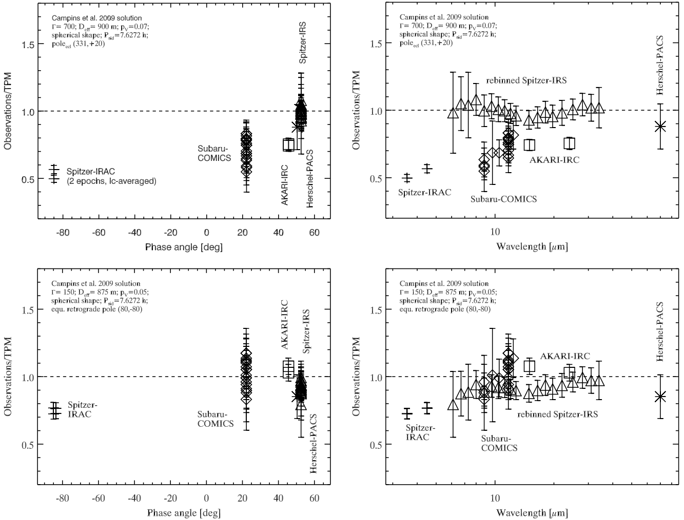
Fig. 10. Test of the Campins et al. (2009) solutions against our large thermal data set. Top left: observation-to-TPM flux ratios as a function of phase angle; top right: as a function of wavelength; bottom: same as top, but now calculated for the lower thermal inertia limit of 150 \text{ J m}^{-2} \text{ s}^{-0.5} \text{ K}^{-1} and the extreme case of an equatorial retrograde geometry (at the time of IRS observations and as seen from Spitzer ).
