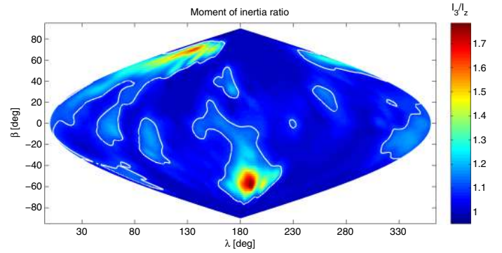
Fig. 5. The colour map of the ratio I_3/I_z for models corresponding to all possible orientations of the spin axis given in ecliptic coordinates (\lambda, \beta) . The white contour corresponds to the level 1.1.
