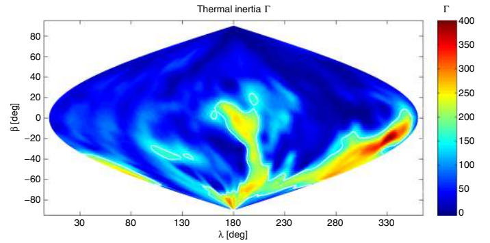
Fig. 6. The colour map of the thermal inertia \Gamma for models corresponding to all possible orientations of the spin axis given in ecliptic coordinates (\lambda, \beta) . The white contour corresponds to \Gamma = 150 \text{ J m}^{-2} \text{ s}^{-0.5} \text{ K}^{-1} .
