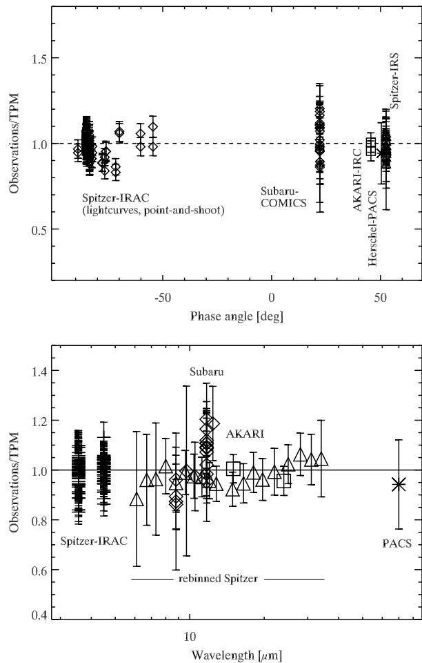
Fig. 12. All thermal observations divided by the corresponding TPM prediction based on solution #2 in Table 5 as a function of phase angle ( top ), and as a function of wavelengths ( bottom ). No trend in observation-to-model flux ratios is visible over the very wide phase angle range from -89^\circ to +53^\circ , nor over the wide range of wavelengths from 3.55 to 70 \mu\text{m} . The rebinned IRS data are shown as triangles together with the absolute flux error of each individual data point.
