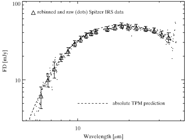
Fig. 14. Absolutely calibrated Spitzer -IRS spectrum from 2nd May, 2008 (see Campins et al. 2009), rebinned data are shown as triangles, the full data set as dots. The absolute TPM prediction (#2 in Table 5) is shown as a dashed line.
