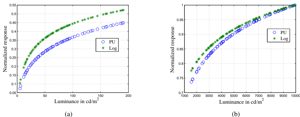
Fig. 2: Comparison of responses for two transformation functions in two different ranges of luminance, (a) 1 - 200 cd/m 2 , (b) 1000 - 10000 cd/m 2 . Figure best viewed in color.
