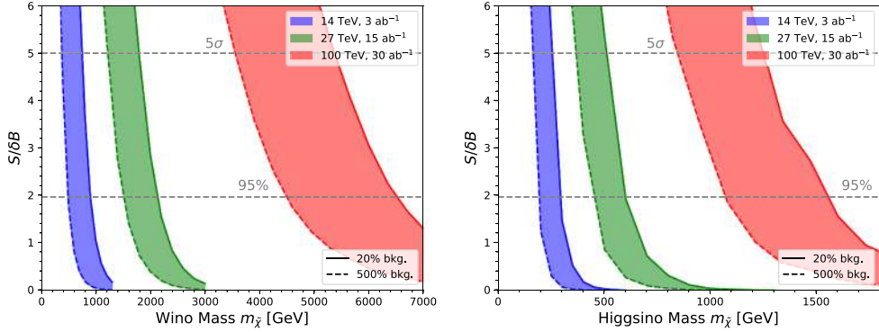
Fig. 1.3. The reach of HE-LHC in the search for a wino (left) or higgsino (right) DM WIMP candidate, using a disappearing charged track signature [17]. The bands limited by the solid and dashed lines show the range obtained by modifying the central value of the background estimate by a factor of five. The results are compared to the reach of HL-LHC and FCC-hh.
