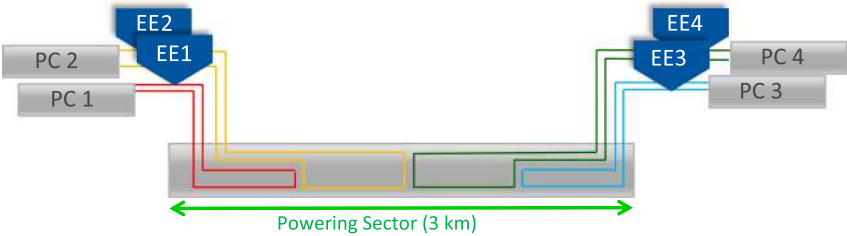
Fig. 3.18. Schematic of the dipole circuit architecture for HE-LHC. Each power converter (PC) is connected to an energy extraction (EE) system.
