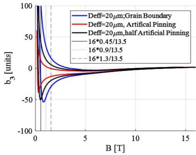
Fig. 3. Sextupolar field error b_3 of the 16 T dipole magnets, in units of 10^{-4} at a reference radius of 16.7 mm, as a function of field strength, for an effective Nb 3 Sn filament size of 20 \mu m, without flux pinning (blue), with 100% artificial pinning (red), and with a realistic 50% pinning efficiency (black). Three different injection energies are indicated.
