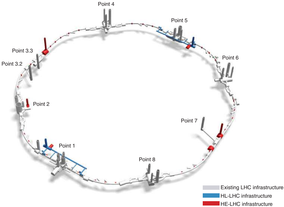
Fig. 4.1. Schematic drawing of the existing LHC underground structures including HL-LHC and HE-LHC upgrades.
