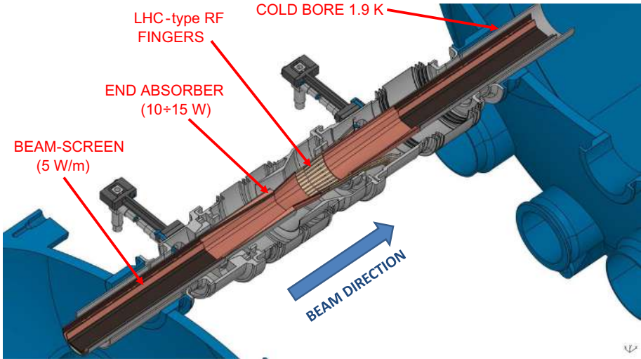
Fig. 3.11. Cut-through, in the plane of the orbit, of the dipole-to-dipole short interconnect area model. This model does not show the BPM block, which is under design in another work package.
