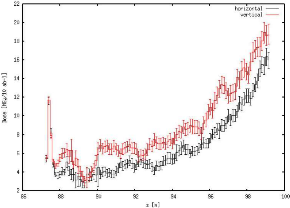
Fig. 2.22. FLUKA simulated peak dose along the separation dipole D1 for a total integrated luminosity of 10\text{ ab}^{-1} and a horizontal (black) or vertical half crossing angle (red) of 165\text{ }\mu\text{rad} , with an inner W shielding of 2 cm.
