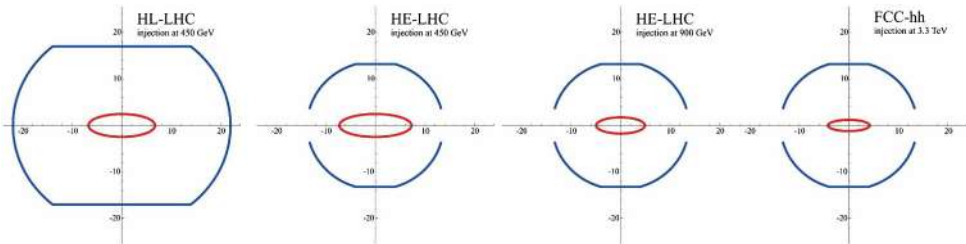
Fig. 2.6. Beam envelope ( 6\sigma ) at injection energy inside the (approximate) beamscreen at a regular arc QF quadrupole for HL-LHC and for HE-LHC with two alternative injection energies (450 and 900 GeV), assuming the 23 \times 90 optics, and for FCC-hh (at 3.3 TeV), without any b_2 field error.
