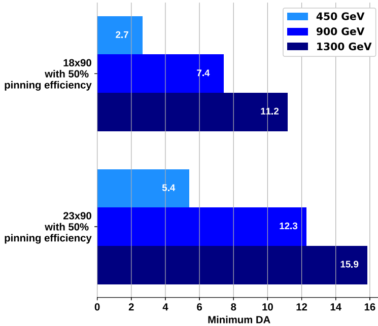
Fig. 2.4. Simulated minimum off-momentum dynamic aperture ( 10^5 turns) due to all non-linear multipole errors, up to 20-poles, assuming 20\text{ }\mu\text{m} Nb 3 Sn filament diameter with 50% flux pinning, as obtained by tracking over 10^5 turns, for 5 angles in x - y space, 60 random error seeds, fractional betatron tunes of 0.28 (H) and 0.31 (V) and a chromaticity Q'_{x,y} corrected to +2 units. These results are a graphical representation of Table 2.4. The systematic part of the b_3 , b_4 and b_5 errors was corrected using one sextupole spool piece next to every main dipole and one nested octupole/decapole spool piece at every second dipole [40].
