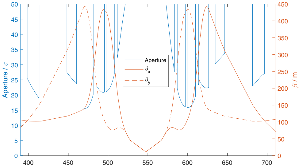
Fig. 2.23. Beta function and apertures for the injection optics at 450 GeV in the experiment IRs 1 and 5, with \beta^* = 11\text{ m} , including a 2 mm closed-orbit uncertainty, with beam–beam separation at the IP and a half crossing angle of 180\text{ }\mu\text{rad} (both separation and angle corresponding to 16.8\sigma ).
