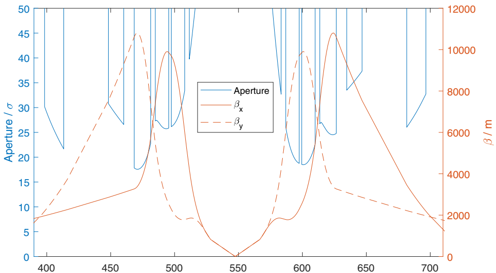
Fig. 2.18. Beta function and aperture for the squeezed optics at collision energy in IRs 1 and 5, for \beta_{x,y}^* = 0.45 m, and a half crossing angle of 165 \mu\text{rad} ( 16.8 \sigma ). The aperture includes a 2 mm closed-orbit uncertainty.
