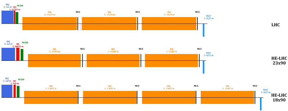
Fig. 2.8. Layout and longitudinal dimensions for the regular arc cell of the present LHC (top), for the HE-LHC 23 \times 90 optics with 23 cells per arc similar to the LHC (centre) and for the alternative HE-LHC 18 \times 90 optics, with 18 cells per arc and longer cells (bottom).
