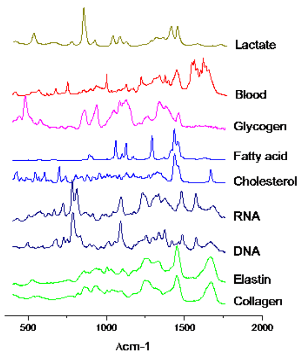
Figure 4 Examples of molecules and their Raman spectrum; (Courtesy of Dr GW Puppels, Erasmus Medical Center, Rotterdam).
