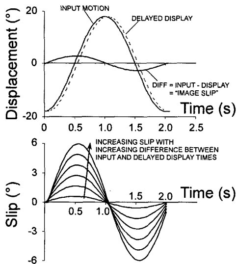
Figure 1. Image slip model for sinusoidal head motion for \pm 18^\circ head yaw at 0.5 Hz with 33 ms base latency plus additional 16.7 ms delay increments. (Top) Because of inherent VE time lag and experimentally added latency, observer input head motion results in delayed motion in the display. The time difference between the input motion and the displayed consequence causes the image slip. (Bottom) The magnitude of the slip grows as the number of added delay steps increases from 0 to 5.
