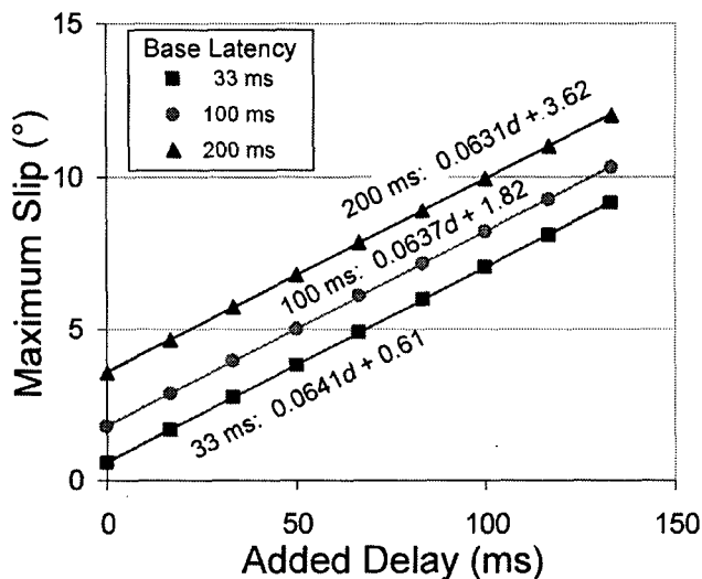
Figure 2. Image slip as a function of time delay for \pm 18^\circ sinusoidal head yaw at 0.5 Hz. Each point marks the maximum slip displacement for 33 ms (lower line), 100 ms (middle line), or 200 ms (upper line) of base latency plus added 16.7 ms delay increments. The regression for each line is of the form Ad + b , where d is the added delay. The slope, A , is approximately equal for all three lines while the intercept, b , changes proportionally to the baseline.
