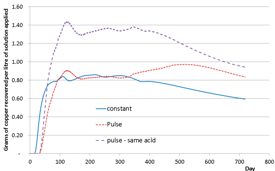
Figure 10. Grams of copper recovered per litre of leaching solution applied.
