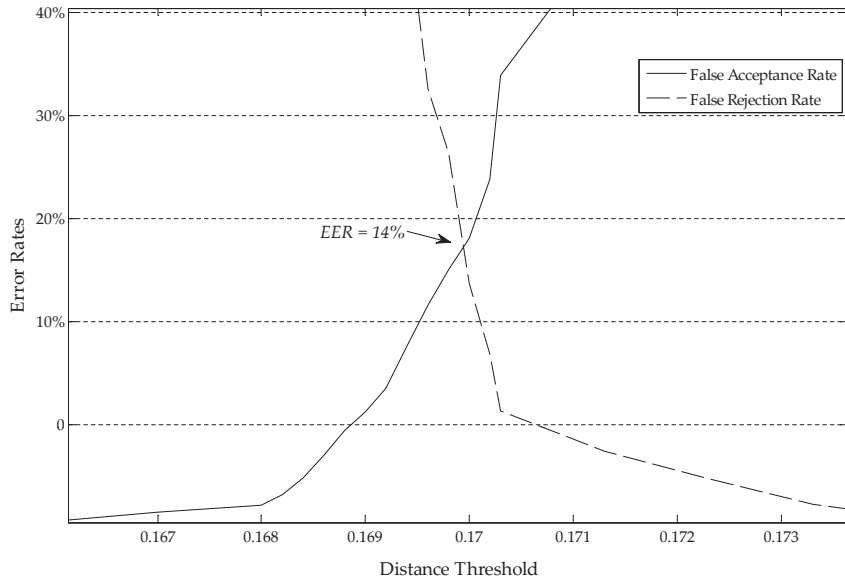
Fig. 5. False Acceptance and Rejection Rates after personalization of the thresholds.
