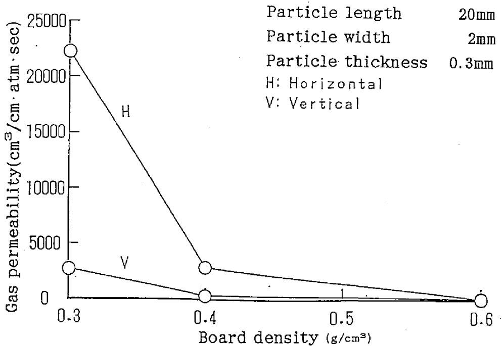
Fig.3.9 Effect of board density on gas permeability of boards.
