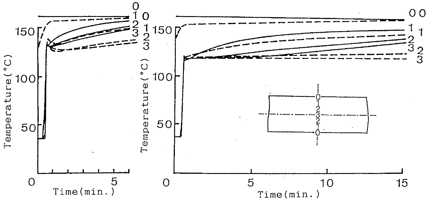
A) Mat density 0.4 g/cm 3 , B) Mat density 0.4 g/cm 3 , Mat thickness 40 mm Mat thickness 20 mm
