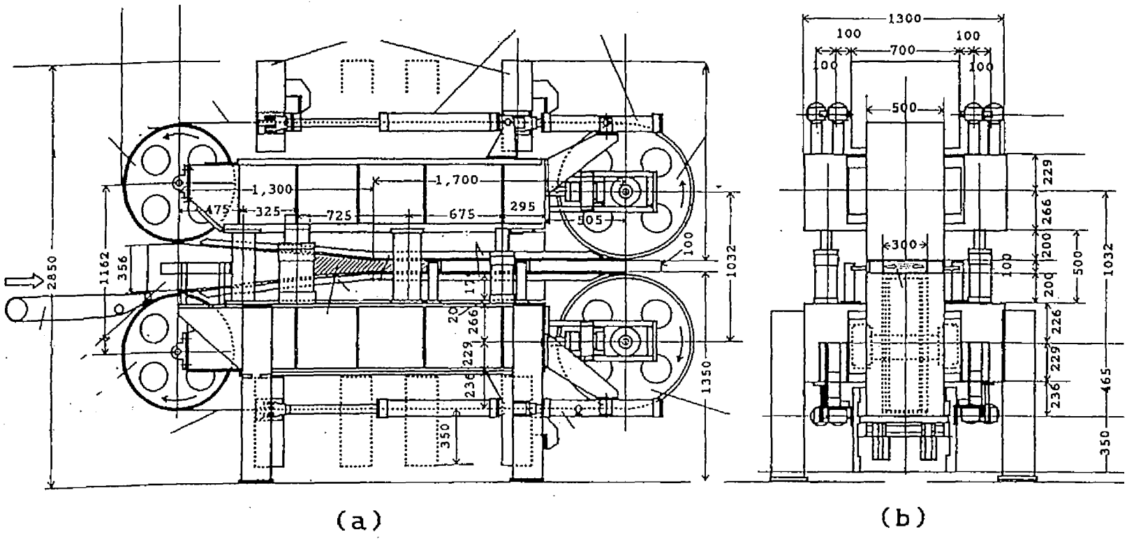
(a) (b) Fig. 1.5 Schematic of Continuous Press with Steam-Injection Heating from Both Sides.
