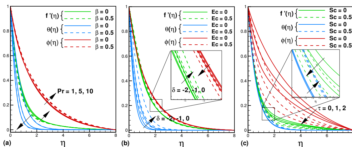
Figure 4: The flow profiles under influences of (a) Prandtl number, (b) heat sink and (c) thermophoresis when \tau = 0.2 , \lambda = M = N = 1 , Pr = 3 , \beta = \gamma = R = Sc = Ec = 0.5 and \delta = -1 respectively.
