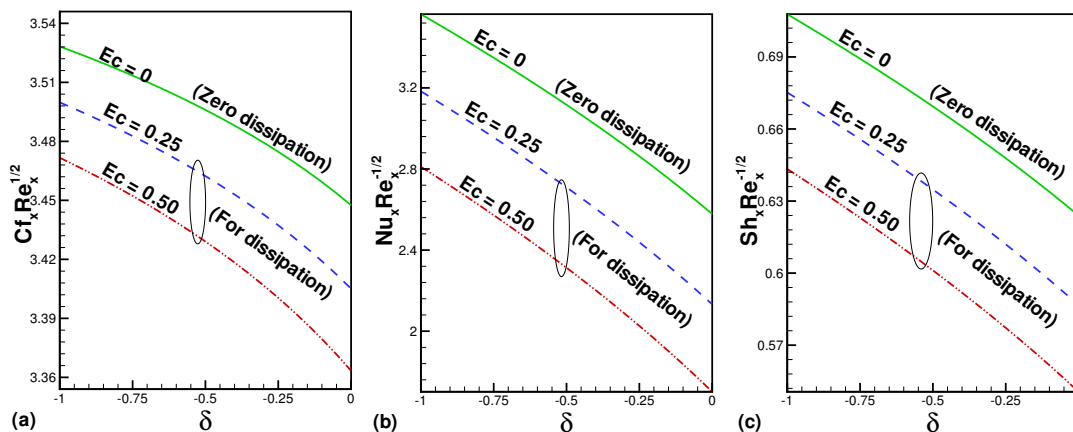
Figure 6: The effects of Eckert number Ec and internal heat sink \delta on (a) reduced skin friction coefficient, (b) reduced Nusselt number and (c) reduced Sherwood number when \beta = \lambda = \tau = M = \gamma = N = R = Sc = 0.5 , Pr = 5 , Sc = 0.25 respectively.
