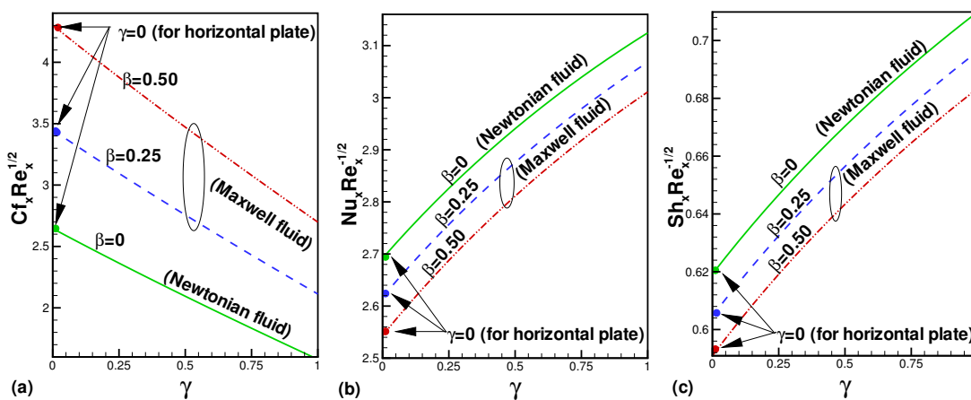
Figure 7: The effects of Maxwell parameter \beta and buoyancy parameter \gamma on (a) reduced skin friction coefficient, (b) reduced Nusselt number and (c) reduced Sherwood number when \beta = \lambda = \tau = M = N = R = Ec = 0.5 , Pr = 5 , Sc = 0.25 , \delta = -1 respectively.
