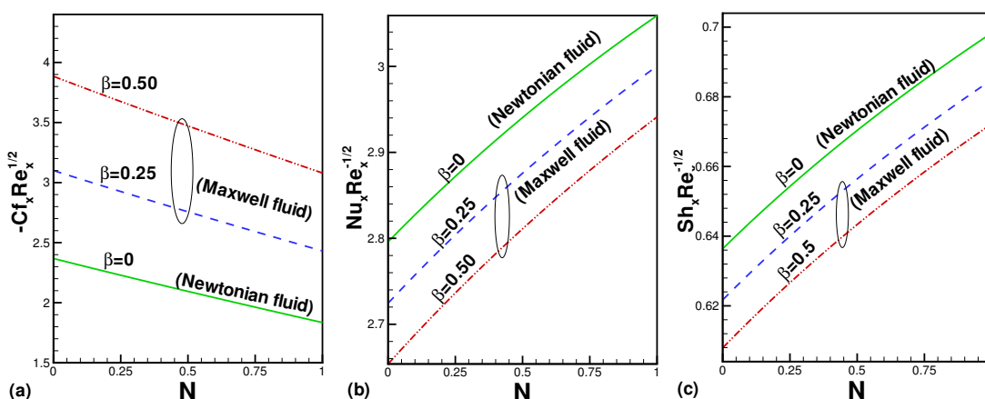
Figure 8: The effects of Maxwell parameter \beta and ratio of volumetric-thermal expansion N on (a) reduced skin friction coefficient, (b) reduced Nusselt number and (c) reduced Sherwood number when \beta = \lambda = \tau = M = \gamma = R = Ec = 0.5 , Pr = 5 , Sc = 0.25 , \delta = -1 respectively.
