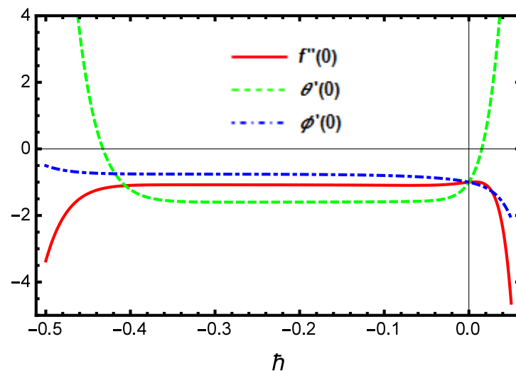
Figure 2: The \hbar curves for f''(0) , \theta'(0) and \phi'(0) using the 20th-order HAM for the case \beta = \tau = 0.2 , M = \lambda = \gamma = N = 1 , \text{Pr} = 3 , Sc = Ec = 0.5 , R = 0.3 and \delta = -1 respectively.
