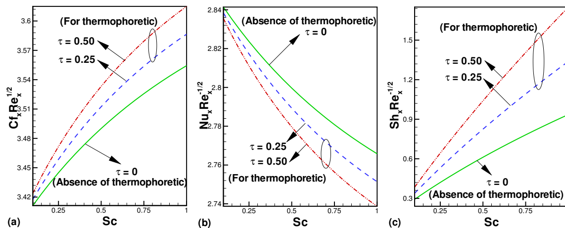
Figure 9: Influence of thermophoresis and Schmidt number Sc on reduced (a) skin friction, (b) Nusselt number and (c) Sherwood number when \beta = M = N = \lambda = \gamma = R = Sc = Ec = 0.5 , Pr = 5 , \delta = -1 respectively.
