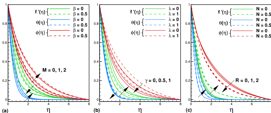
Figure 3: The flow profiles under influences of (a) Hartmann number, (b) buoyancy and (c) thermal radiation when \tau = 0.2 , \beta = R = 0.3 , \lambda = \gamma = 1 , Pr = 3 , M = N = Sc = Ec = 0.5 and \delta = -1 respectively.
