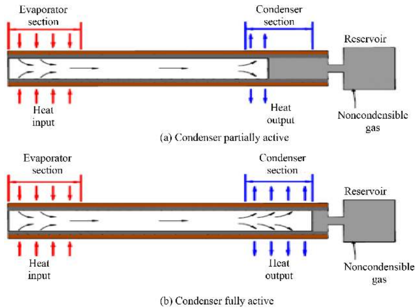
Figure 6. Variable conductance heat pipe.
