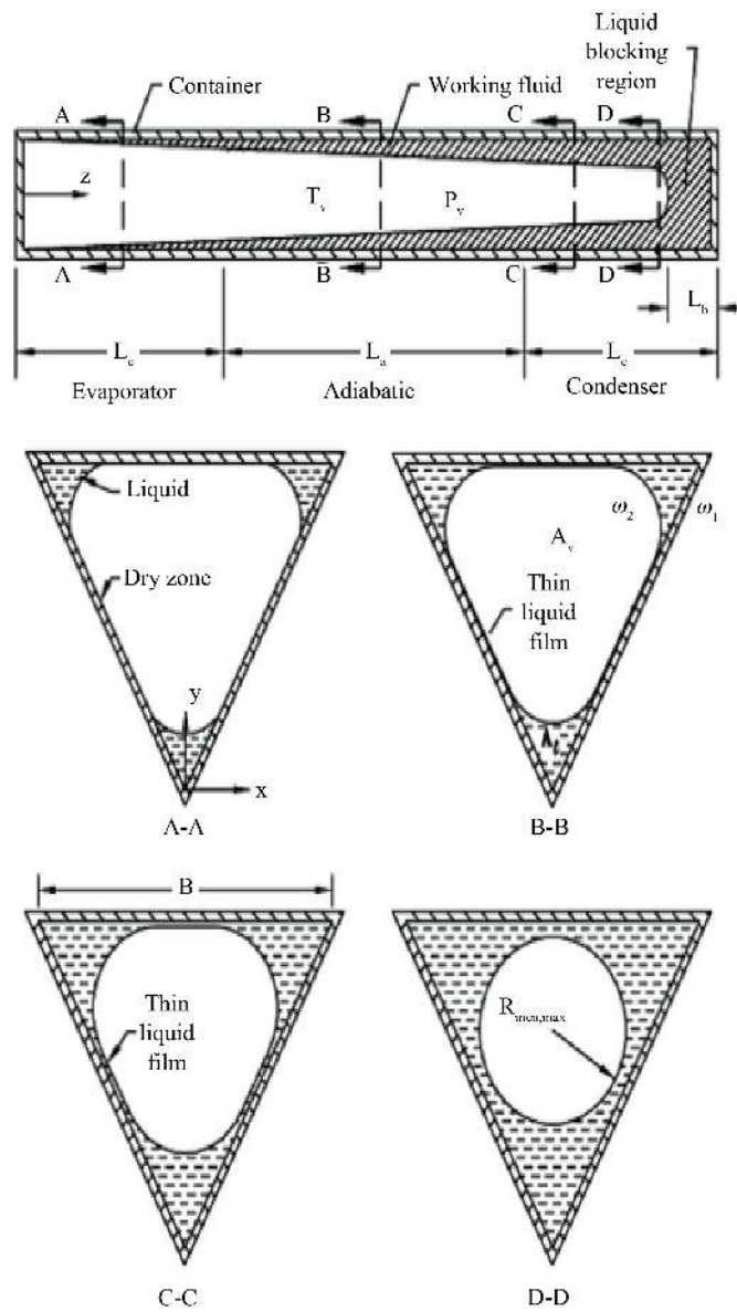
Figure 9. Schematic of Micro heat pipe.
