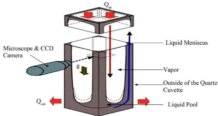
Figure 3. Constrained vapor bubble experiment for international space station.
