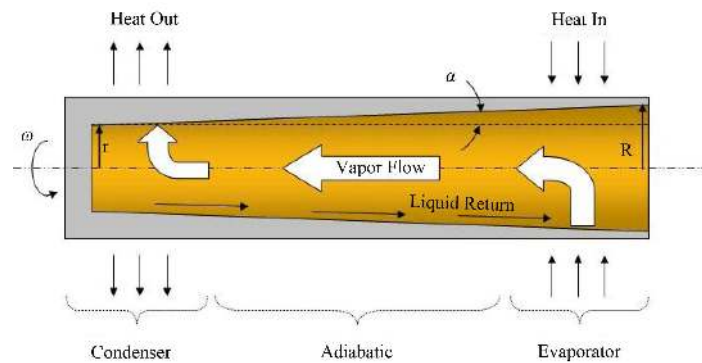
Figure 8. Flow mechanism in a rotating heat pipe.
