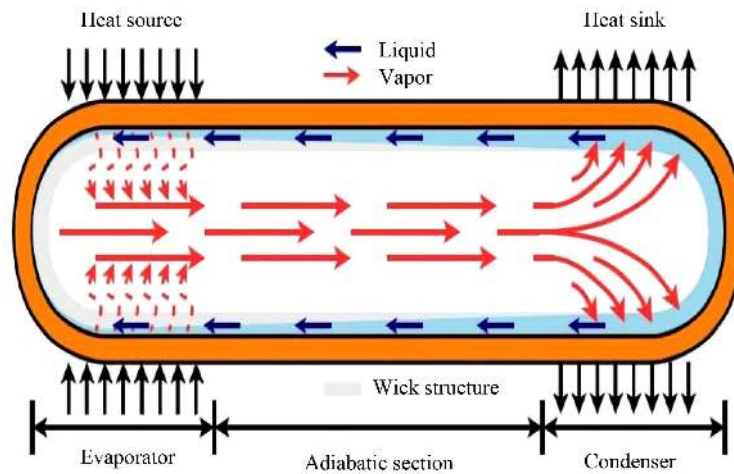
Figure 1. Schematic of a heat pipe.
