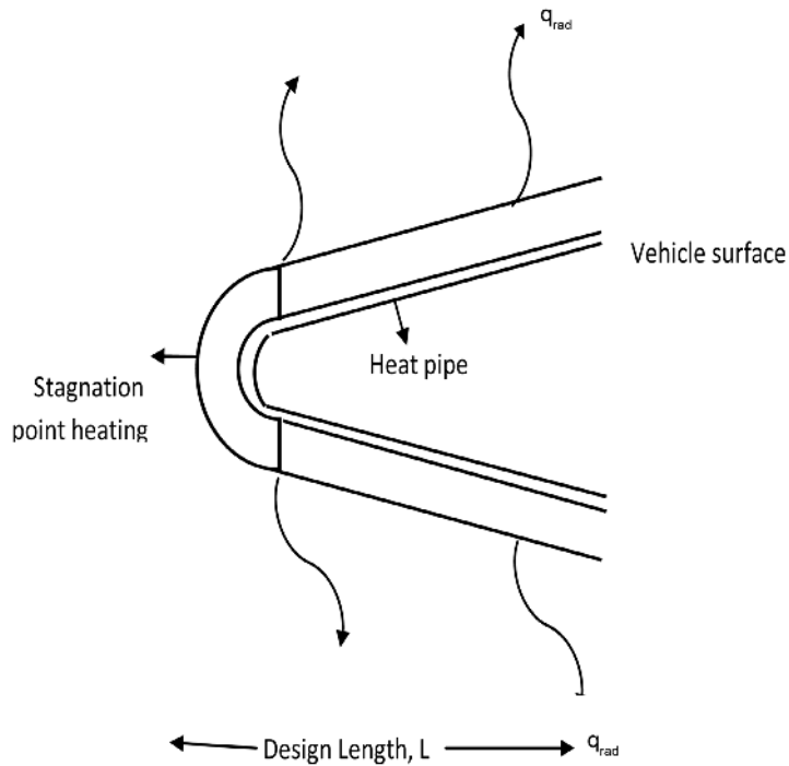
Figure 2. The local geometry and flow conditions near the leading edge.
