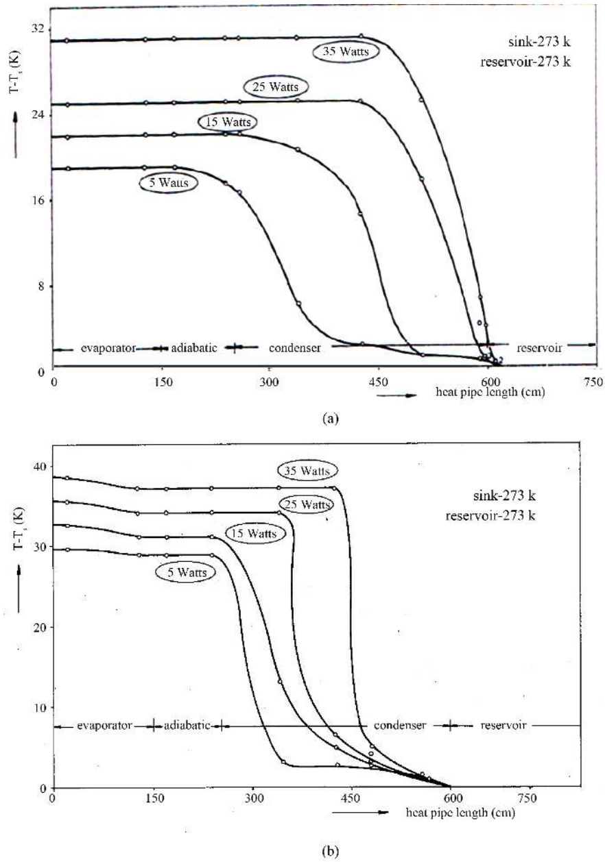
Figure 7. Wall Temperature along methanol VCHP with Control gas (a) NH 3 , (b) N 2 , [30].
