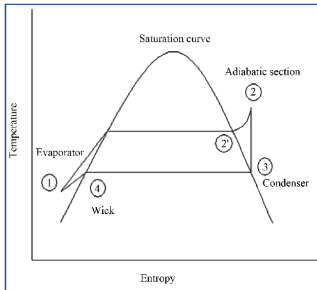
Figure 4. Thermodynamic operation of heat pipe.
