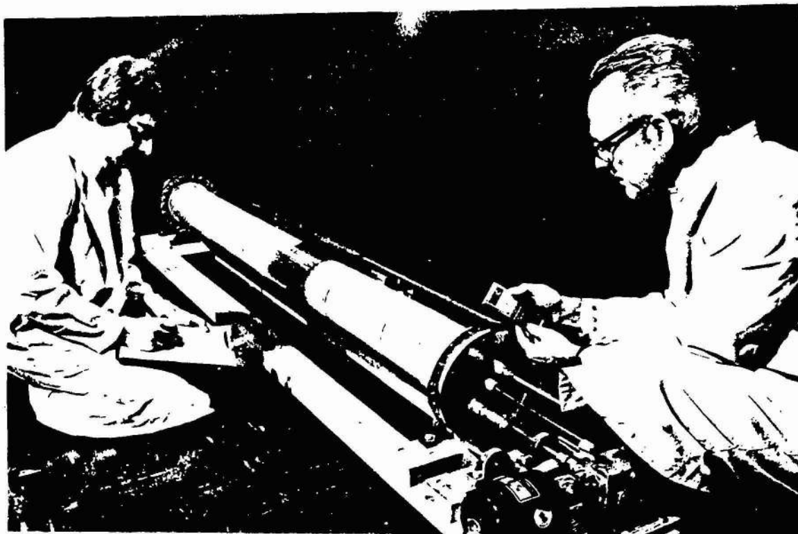
Figure 10 The Axial Solids Transport Experiment Demonstrated Uniform Freezing in Long Cylinders
