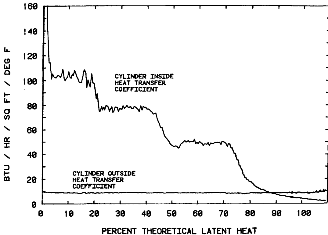
Figure 7 Heat Transfer Coefficients for Run 44, 3 RPM, 25% Excess Na 2 SO 4 , Cycle 10
