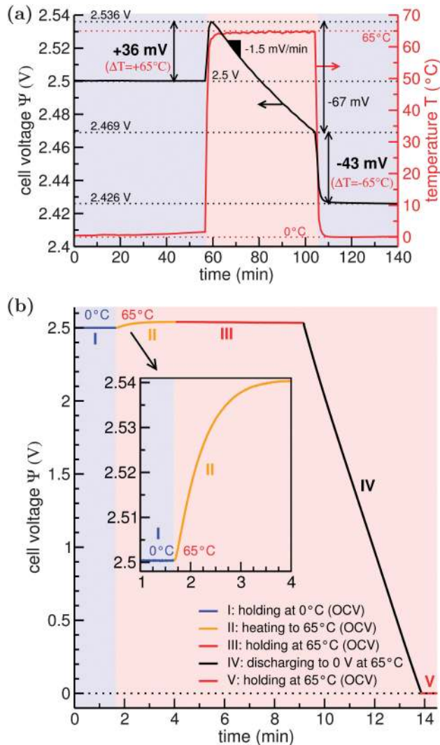
Fig. 2 (a) Open circuit potential measurements when cycling the fully charged cell between 0^\circ\text{C} and 65^\circ\text{C} . We kept the device at each temperature for about 40 minutes to clearly present the effect of self-discharge at the respective temperatures (almost zero at T = 0^\circ\text{C} and around -1.5 \text{ mV min}^{-1} at T = 65^\circ\text{C} ). (b) Full half-cycle measurement of the thermal voltage rise (I \rightarrow III) and discharging to 0 V (III \rightarrow V). Again, steps I, III, and V just show that the open circuit potential stays almost constant in the respective states. For application this time can be reduced to a minimum.
