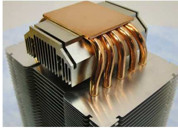
Fig. 3: Heat Pipes Cooler with Aluminum Fins
