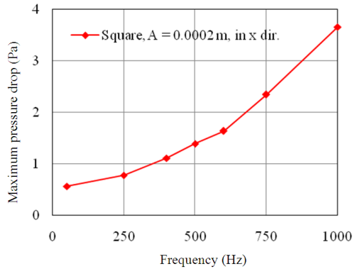
Fig. 6: Effect of Frequency on Maximum Pressure Drop for 2D Square Pin Fin (Gururatana, 2011)
