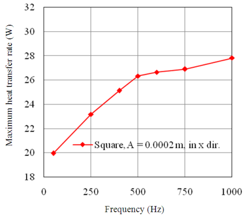
Fig. 5: Effect of Frequency on Maximum Heat Transfer for 2D Square Pin Fin (Gururatana, 2011)
