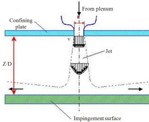
Fig. 2: Confined Jet Impingement
