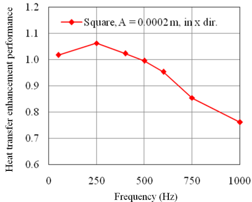
Fig. 7: Effect of Frequency on Heat Transfer Enhancement Performance for 2D Square Pin Fin (Gururatana, 2011)
