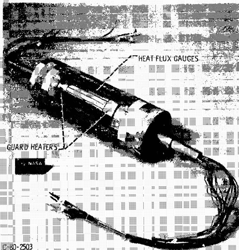
Figure 3 - Cylinder heat transfer model.
