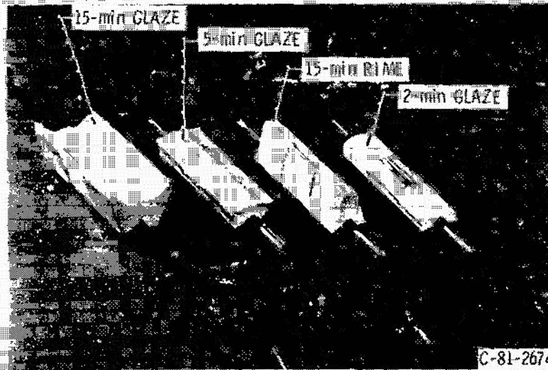
Figure 2 - Photograph of ice rig shape heat transfer models.
