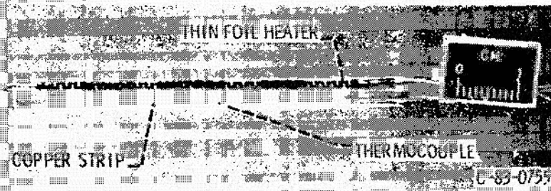
Figure 4 - Photograph of heat flux gauge.
