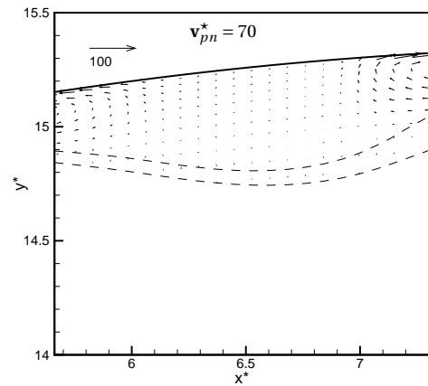
(b) P'^* = 4.0 , \dot{m}'_p = 0.7 and U^* = 2.0
