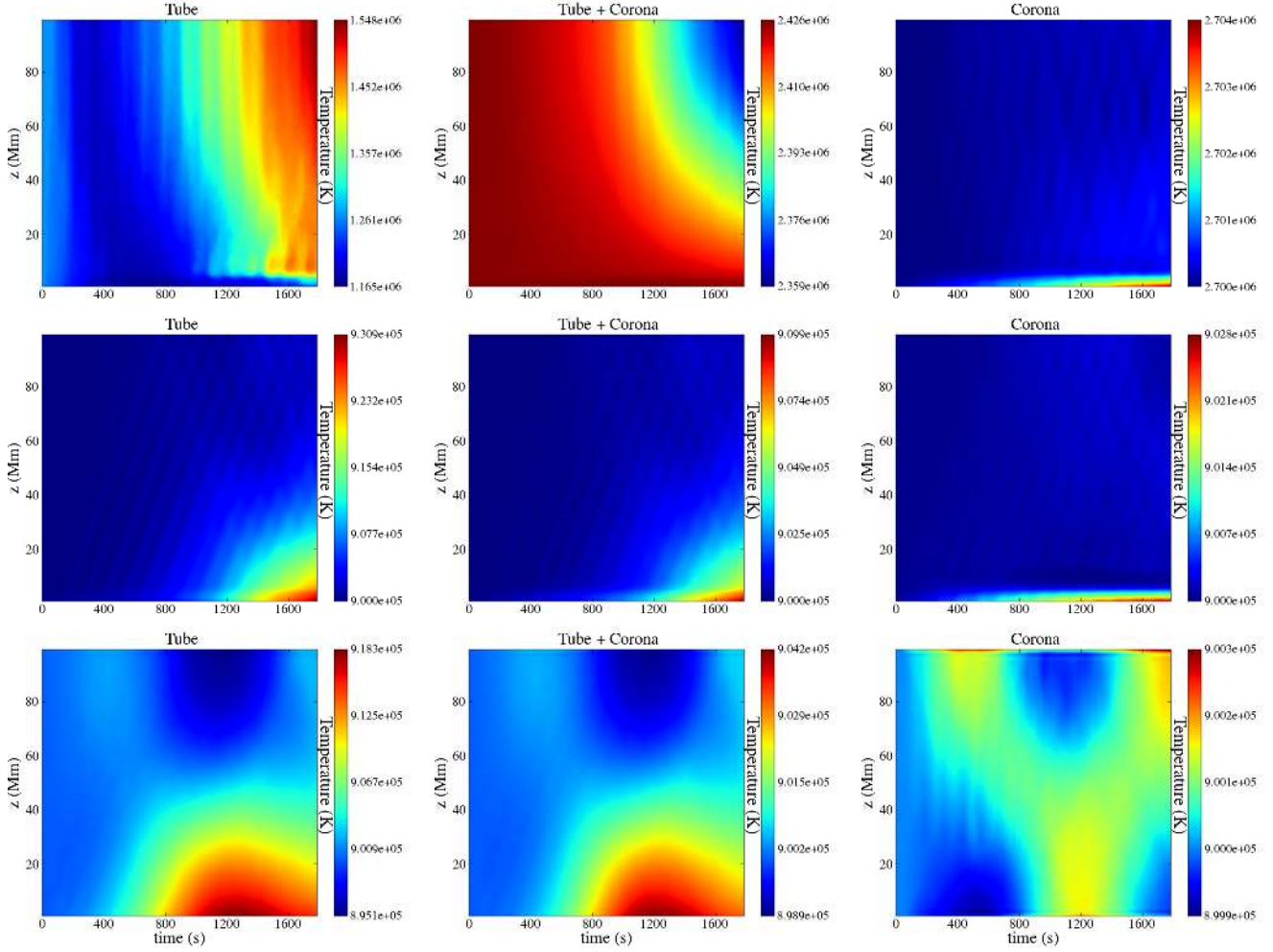
Fig. 8. Average temperature along the z -axis: ( left ) inside the tube (for \rho \geq 0.84 \times 10^{-12} \text{ kg m}^{-3} ), ( centre ) for the whole greater region (tube+corona) including the loop ( 0 \leq z \leq 100 \text{ Mm} , |x| \leq 2.33 \text{ Mm} and y \leq 2.33 \text{ Mm} ) and ( right ) for the surrounding plasma outside the loop. From top to bottom: a) the Driven-diffT model; b) the Driven-equalT model and c) the Stand-equalT model. The apex is located at z = 100 \text{ Mm} .
