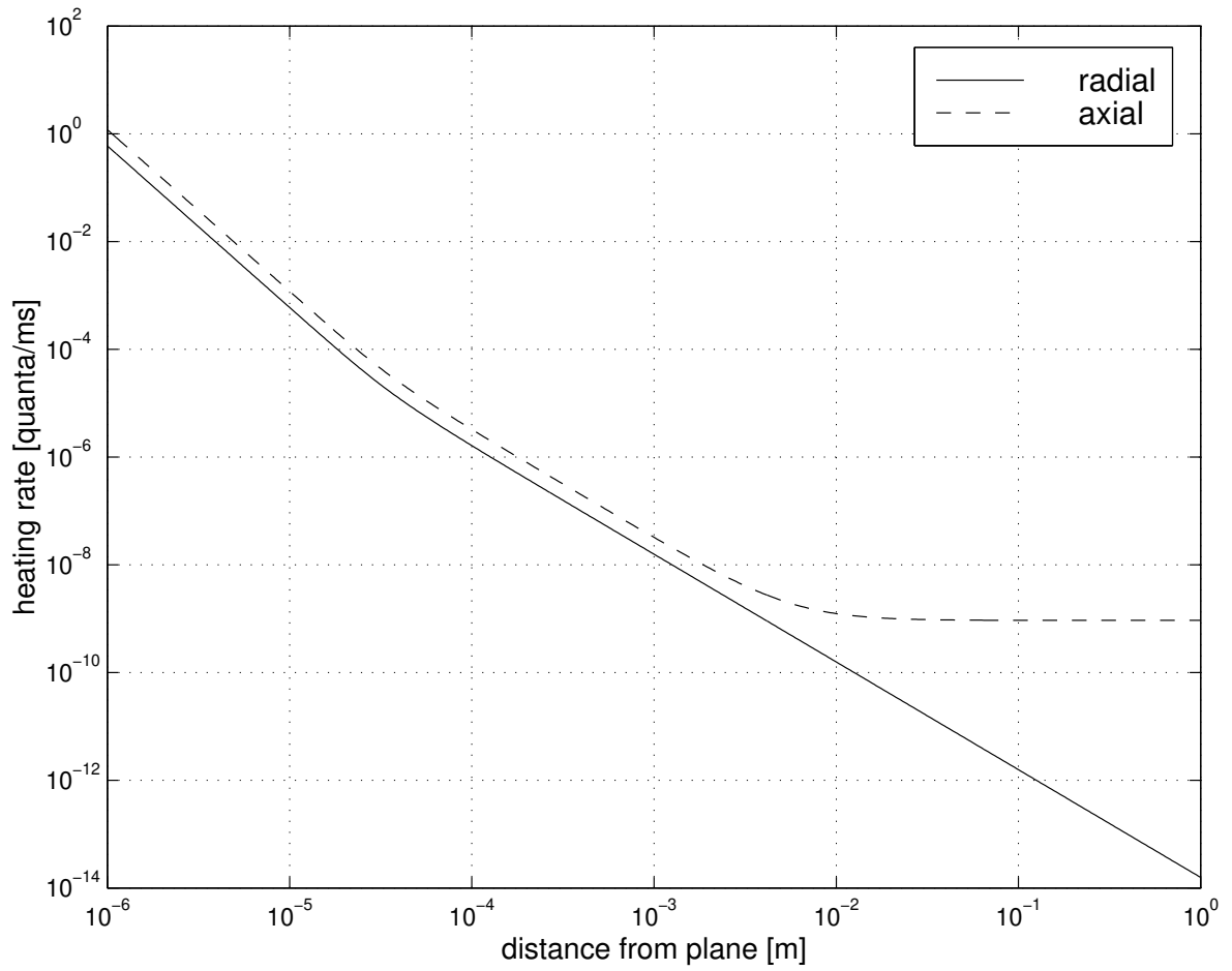
FIG. 7. Expected heating rate vs. distance from electrode for thermal electronic noise, from Eqs. (17), (18) and (4). The numerical parameters are those for {}^9\text{Be}^+ with molybdenum electrodes at 10 MHz secular frequency and room temperature.
