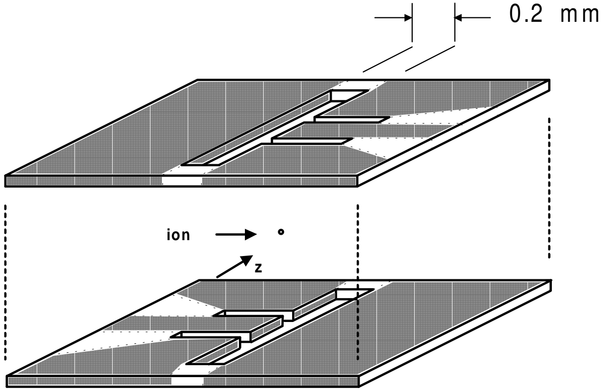
FIG. 3. Schematic diagram of the electrodes of the linear traps (traps 4, 5 and 6 from Table I). The traps are formed by evaporating gold (approximately 0.75 \mu\text{m} thick) on an alumina substrate. The outer segmented electrodes are the endcaps, while the long unbroken electrodes carry rf. The axial direction (labeled z ) is parallel to the rf electrode. The two separate trap wafers are spaced by 200 \mu\text{m} for traps 4 and 5 and 280 \mu\text{m} for trap 6 (spacers not shown). Schematic diagram not to scale.
