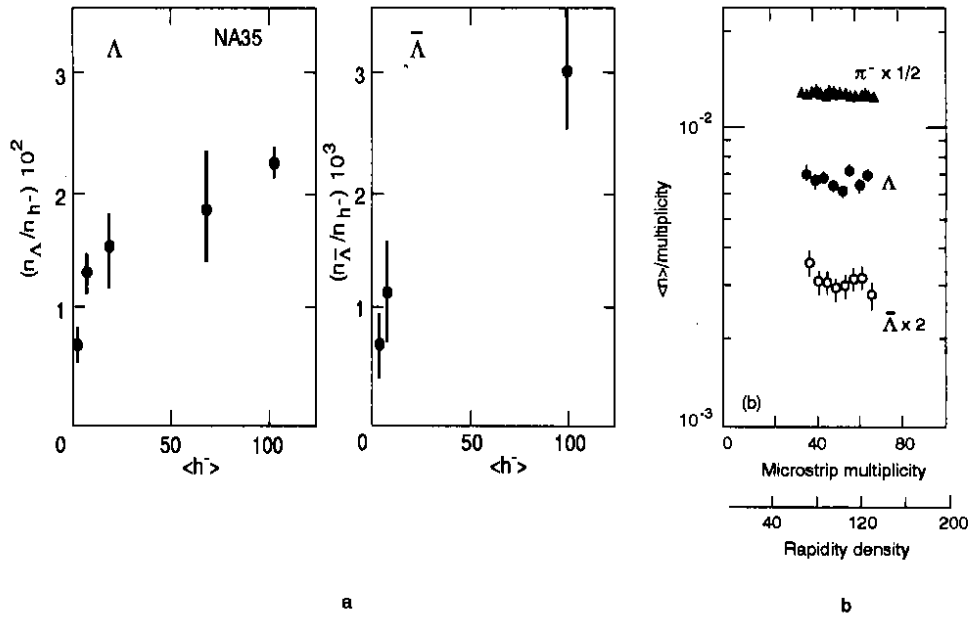
Figure 2: Hyperon and antihyperon yield normalized to negative production. a.) Results from NA35 in sulfur-sulfur collisions. b.) Results from WA85 in sulfur-tungsten collisions ( 2.3 < y_{lab} < 3.0 ).
