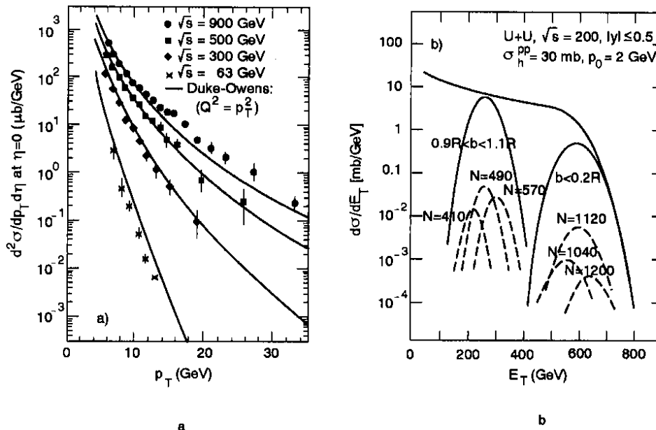
Figure 4: Minijets at the origin of quark-gluon plasma formation at RHIC energy. a) The inclusive jet yield and QCD prediction. b) The transverse-energy yield in UU collision expected from minijets down to 2 GeV/c.
