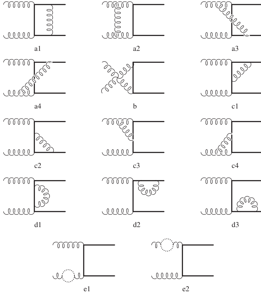
FIG. 3. The t -channel one-loop graphs contributing to the gluon fusion amplitude. Loops with dotted lines represent the gluon, ghost, and light and heavy quarks.
