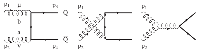
FIG. 2. The t -, u -, and s -channel LO graphs contributing to the gluon (curly lines) fusion amplitude. The thick solid lines correspond to the heavy quarks.
