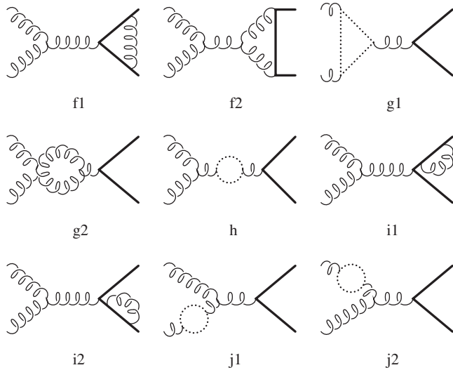
FIG. 4. The s -channel one-loop graphs contributing to the gluon fusion amplitude. Loops with the dotted lines as in g1, h, j1, and j2 represent the gluon, ghost, and light and heavy quarks. The four-gluon coupling contribution appears in g2.
